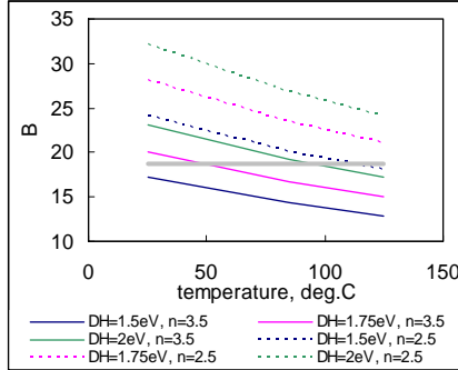
Figure 9. Variations of parameter B with temperature for n = 2.5 and 3.5 and activation energies \Delta H = 1.5\text{ eV} , 1.75\text{ eV} , and 2\text{ eV} . A horizontal line corresponds to the value of B used in MIL-PRF-55365.
