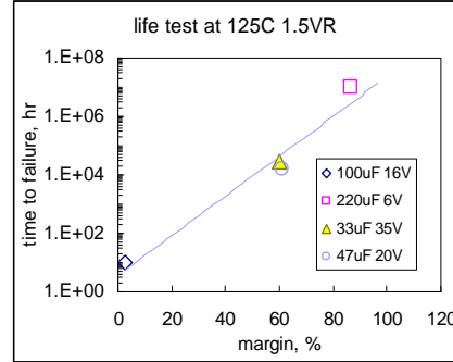
Figure 10. Variations of the characteristics time to failure obtained during highly accelerated testing of four part types at 125^\circ\text{C} , 1.5\text{ VR} with the safety margin.
