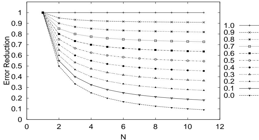
Figure 1: Effect of correlation and number of base classifiers on error reduction. Each line represents a particular average correlation indicated in the legend on the right.
