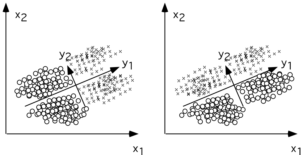
Figure 2: PCA and classification: The first principal component ( y_1 ) can provide a good discriminating feature (left) or a poor one (right), since the class membership information is not used.
