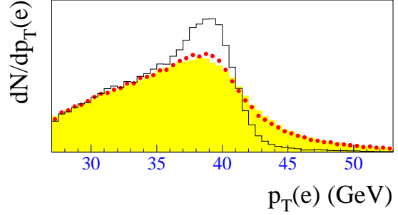
Figure 1. The effects of resolution and the finite p_T^W on p_T^e in W boson decay. The histogram shows p_T^e without detector smearing and for p_T^W = 0 . The dots include the effects of adding finite p_T^W , while the shaded histogram includes the effects of detector resolutions. The effects are calculated for the DØ Run I detector resolutions.
