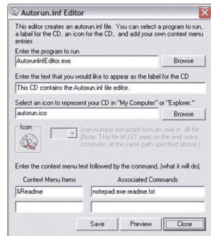
Figure 2: Autorun.inf Editor
