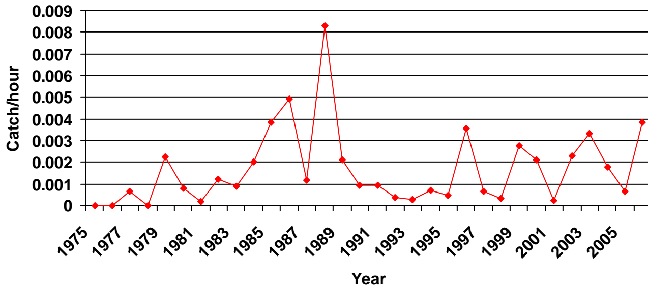
Figure 5. 1975-2006 coastwide gill net CPUE (number/hour) of Atlantic sharpnose sharks.
