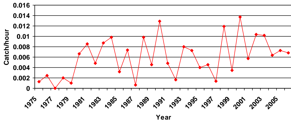
Figure 4. 1975-2006 coastwide gill net CPUE (number/hour) of bonnethead sharks.
