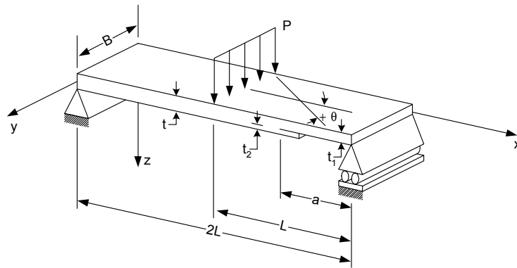
FIGURE A-1. THE SINGLE LEG BENDING TEST
