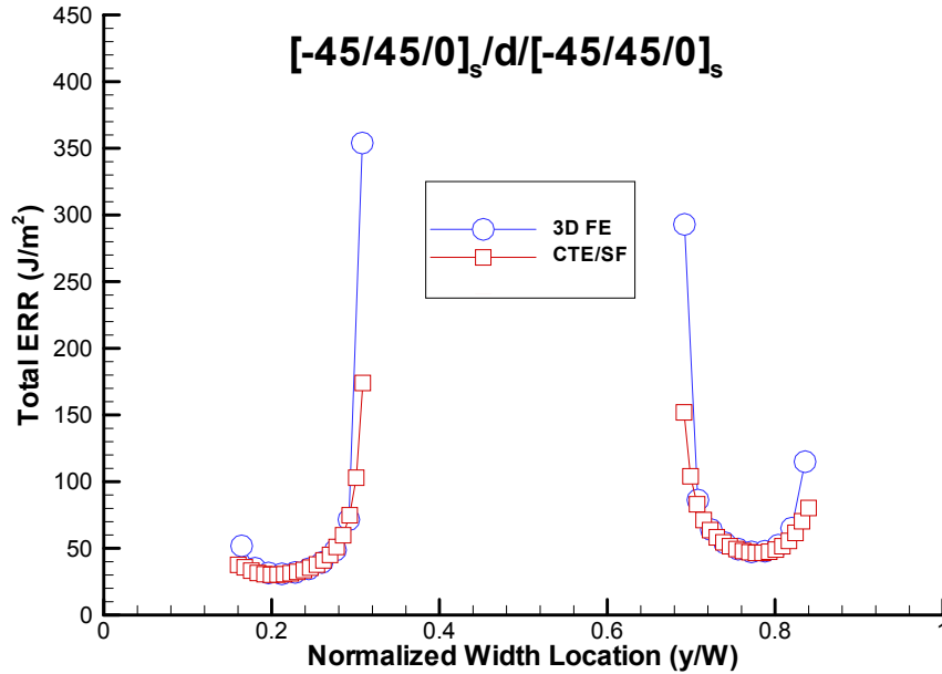
FIGURE 23. COMPARISON OF TOTAL ERRs FOR A [-45/45/0]_s/d/[-45/45/0]_s HAT-STIFFENED PANEL
