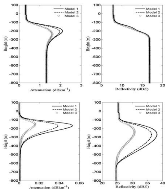
Figure 2. Simulated profiles of radar reflectivity and attenuation at (top) 94 GHz and (bottom) 3 GHz for three different models of melting snowflakes (Fabry and Szyrmer, 1999) for a Marshall-Palmer raindrop size distribution and 1\text{ mmhr}^{-1} surface rainfall rate.
