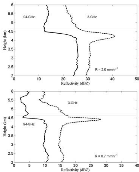
Figure 1. Observed profiles of radar reflectivity at 3 GHz (dotted line) and 94 GHz (solid line) in stratiform precipitation. The 0^{\circ}\text{C} isotherm is located at 4.6 km and the surface rainfall rate is (top) 2\text{ mmhr}^{-1} and (bottom) 0.7\text{ mmhr}^{-1} . The 94 GHz radar reflectivity profile below the melting layer (only raindrops) has been corrected for Mie effects and attenuation using the corresponding 3 GHz radar reflectivity values and offset for clarity.
