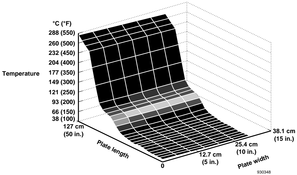
Figure 4. Typical temperature profile and division of the test plate into strips.
