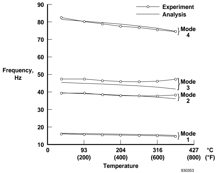
Figure 9. Comparison of analytical and experimental frequencies for a uniformly heated titanium plate.
