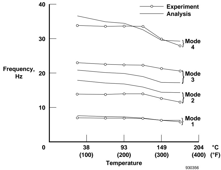
Figure 12. Comparison of analytical and experimental frequencies for fiberglass plate #1 at a uniform temperature profile.
