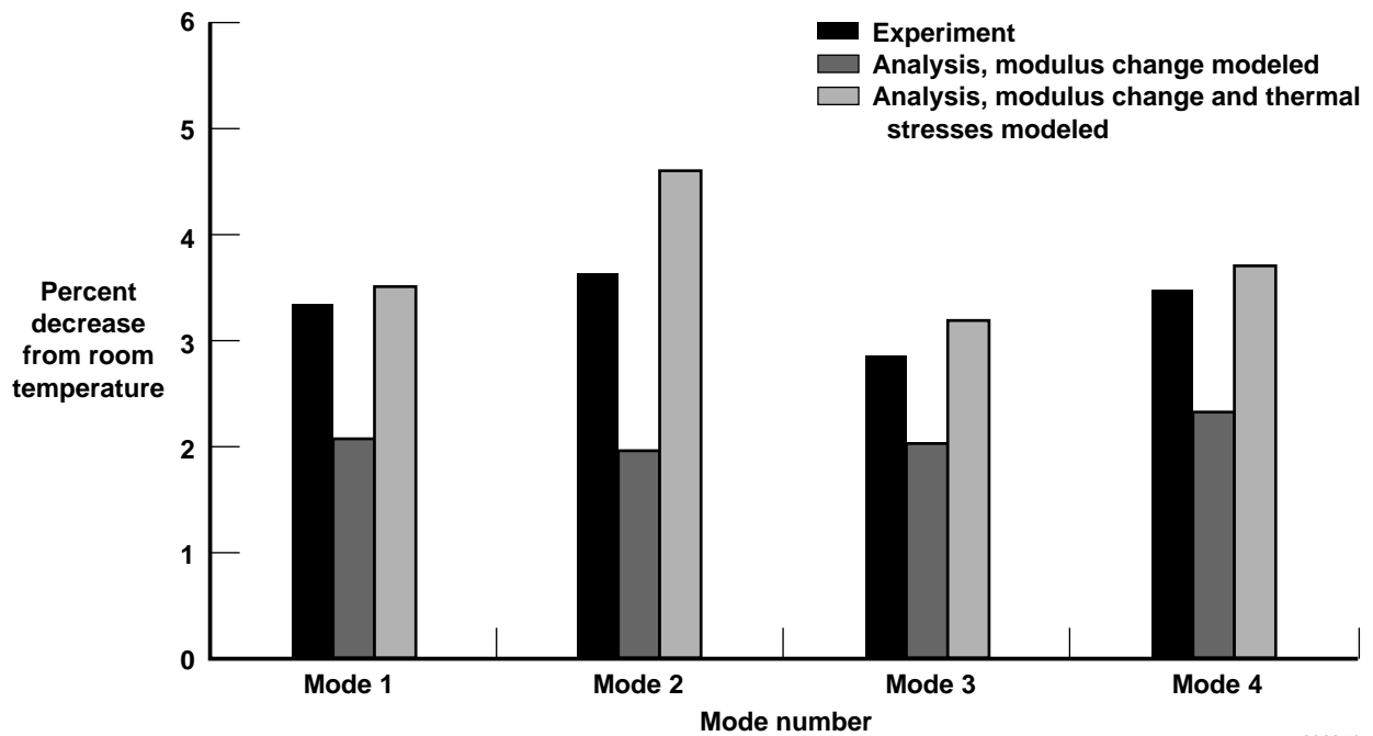
Figure 7. Comparison of analytical and experimental frequency changes for a nonuniformly heated aluminum plate.
