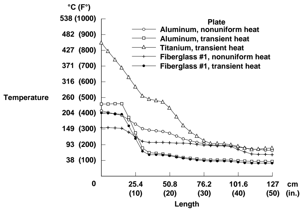
Figure 3. Plate temperature distributions for nonuniform and transient heating profiles.
