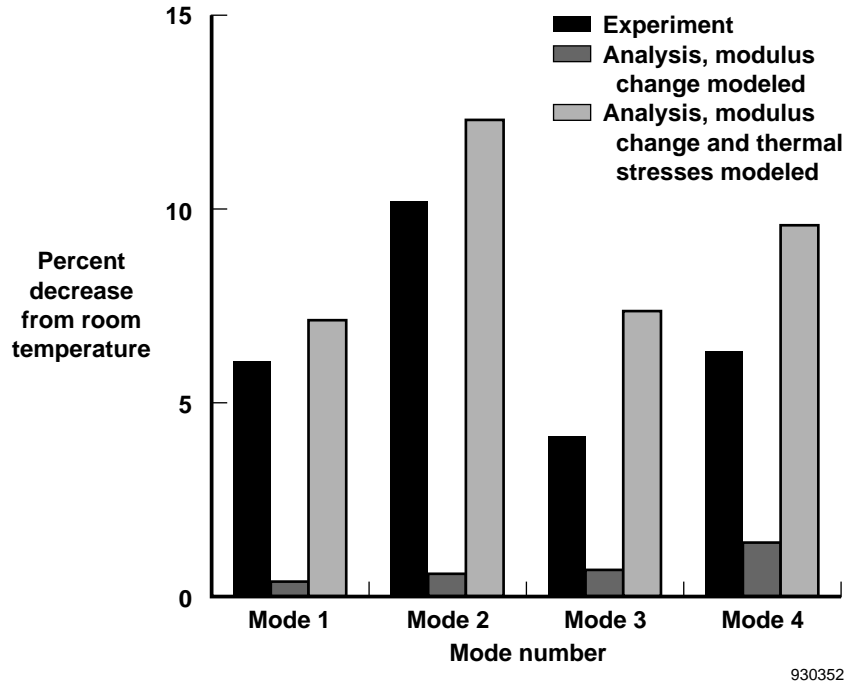
Figure 8. Comparison of analytical and experimental frequency changes for a transiently heated aluminum plate.
