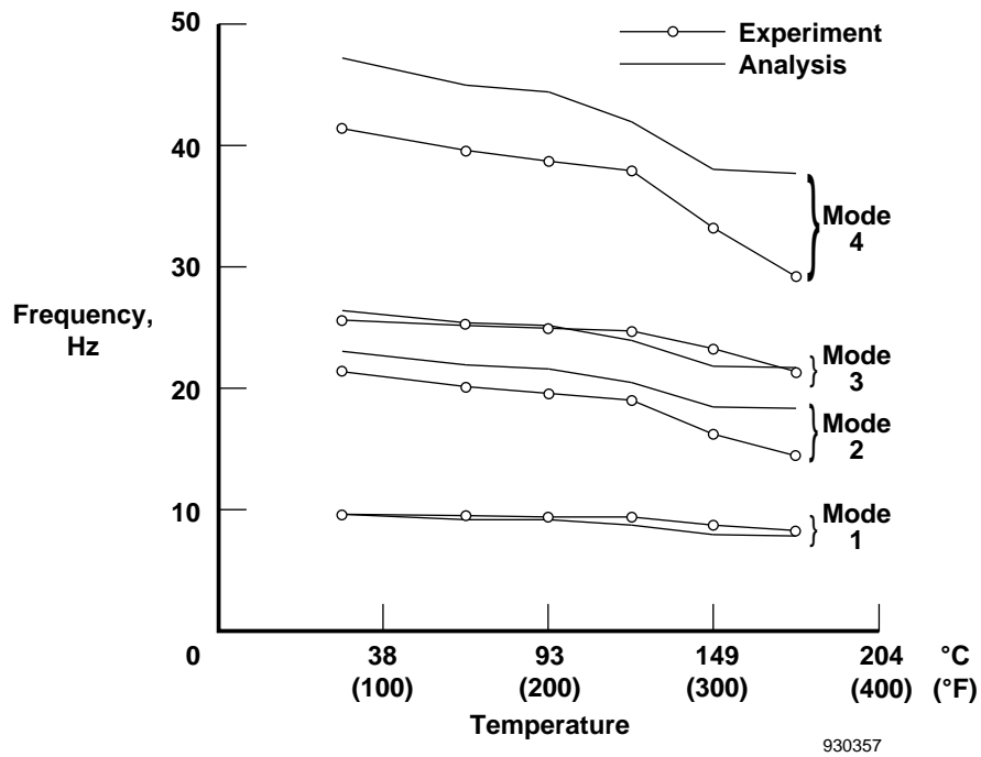
Figure 13. Comparison of analytical and experimental frequencies for fiberglass plate #2 at a uniform temperature profile.
