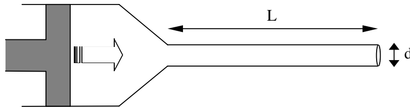
Fig. 6. Diagram of a simple extrusion viscometer.
