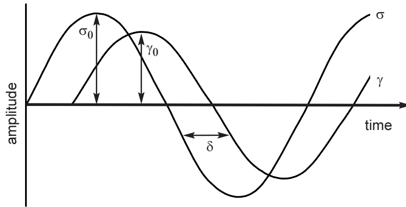
Fig. 3. Sinusoidal wave forms for stress and strain functions.
