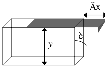
Figure 1 Shear strain schematic.
