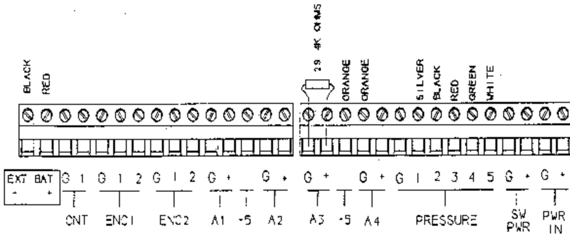
(B) 8200 Terminal Strip
