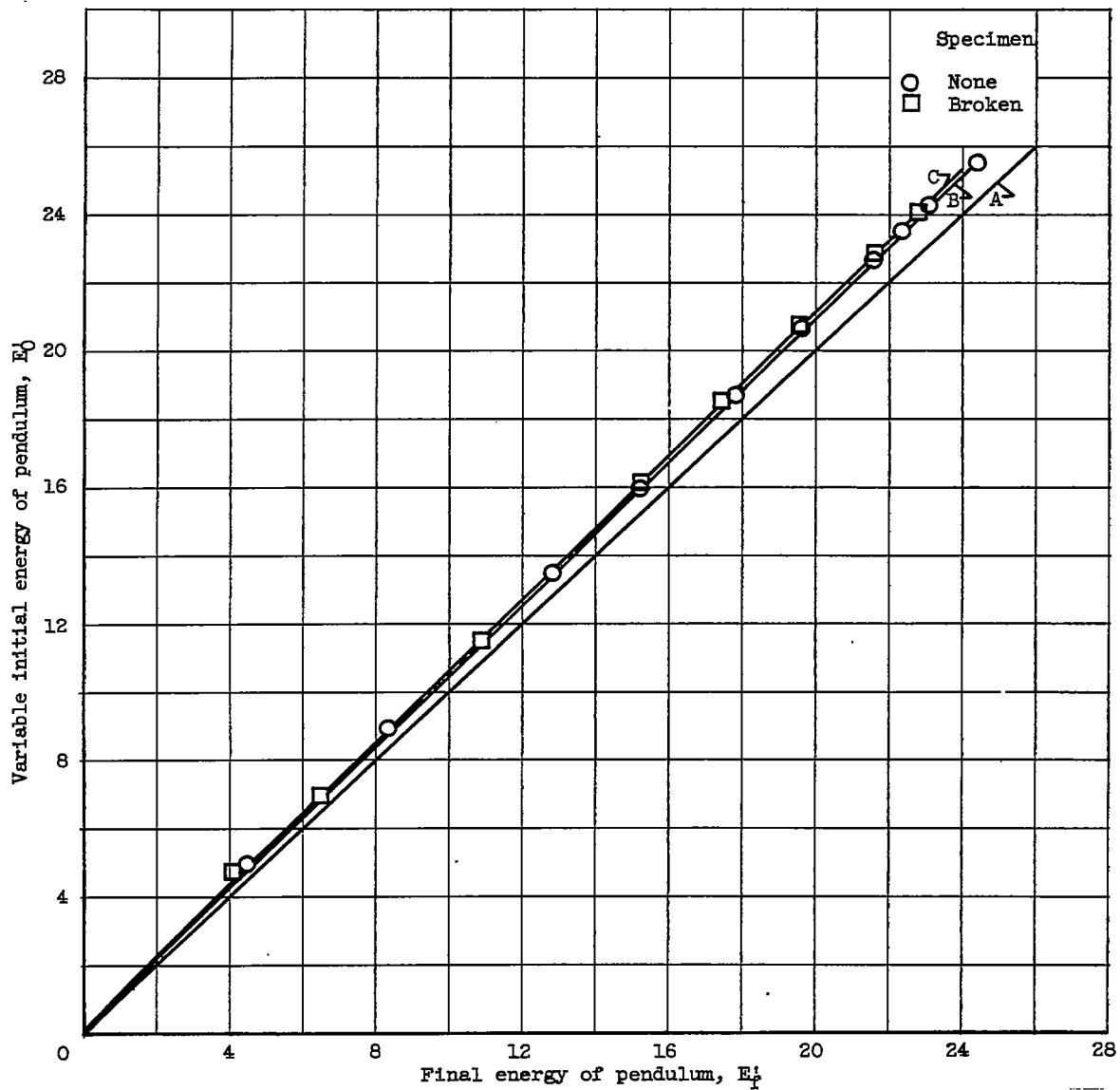
Figure 4. - Experimental curves relating initial and final energies of pendulum for K152B.
