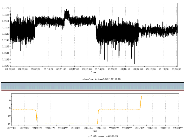
Figure 7. Tune shift during and after sextupole correction. Notice in Figure 6 and 7 a variation in the resolution of the PLL tune data. The primary factor influencing PLL
