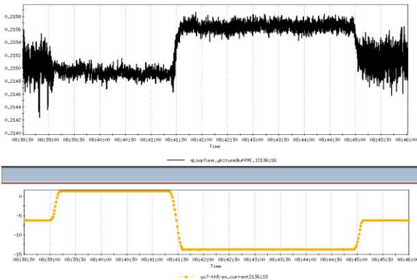
Figure 6. Tune shift vs. bump amplitude after octupole correction.
