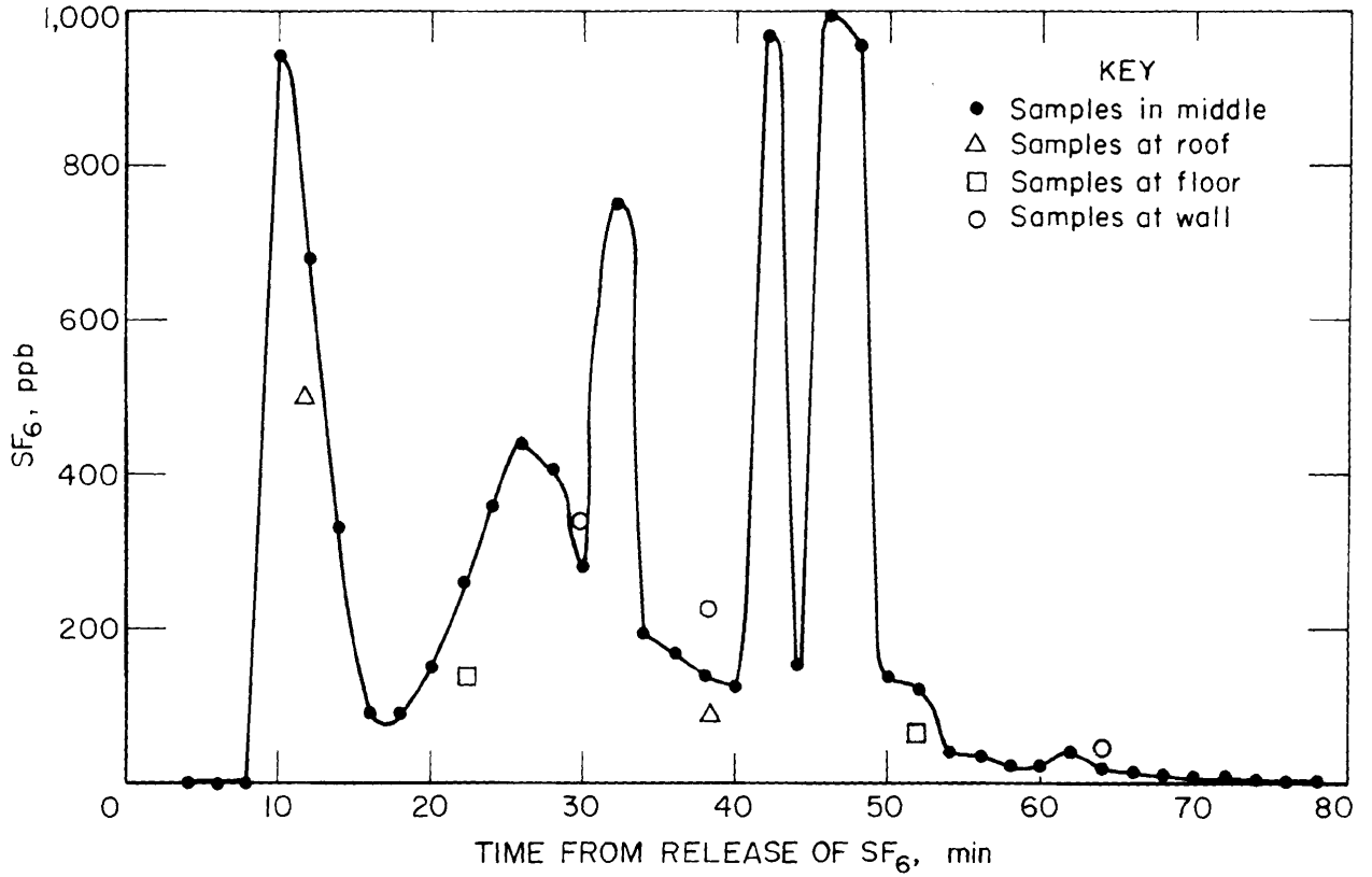
FIGURE 1. - SF 6 concentration as a function of time for a case of poor mixing.
