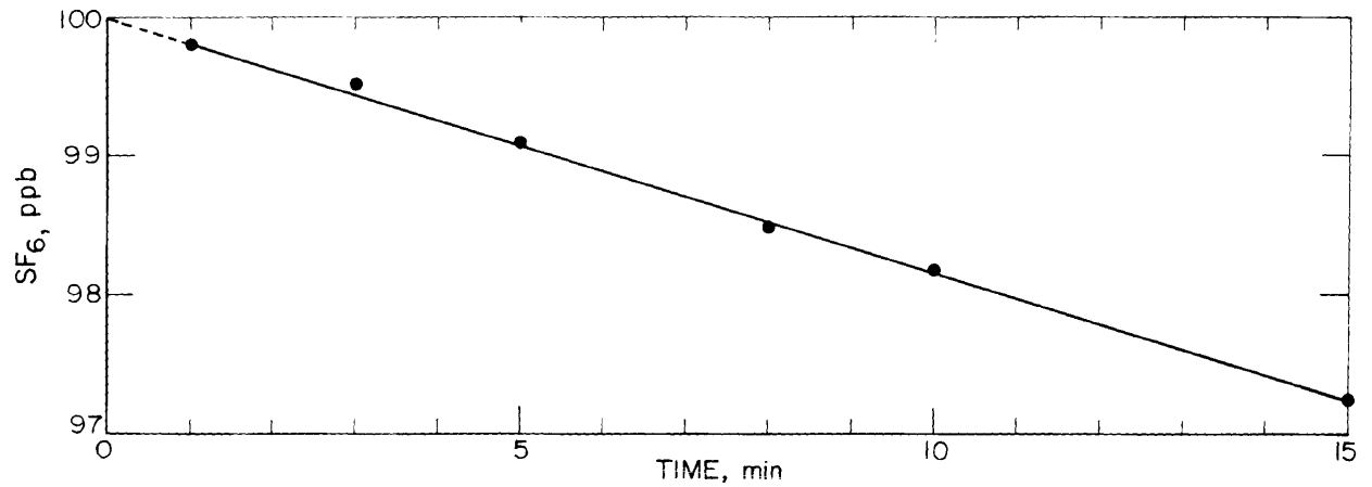
FIGURE 5. - SF 6 concentration in a room as a function of time.
