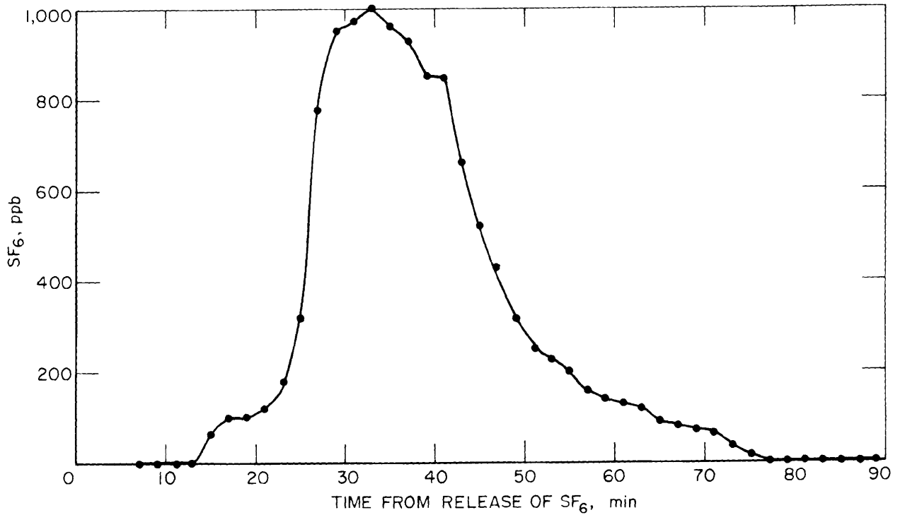
FIGURE 2. - SF 6 concentration as a function of time for a case of good mixing.
