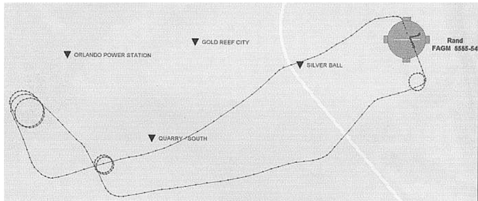
Figure 4 - Typical flight path for SWIS Phase I tests.
