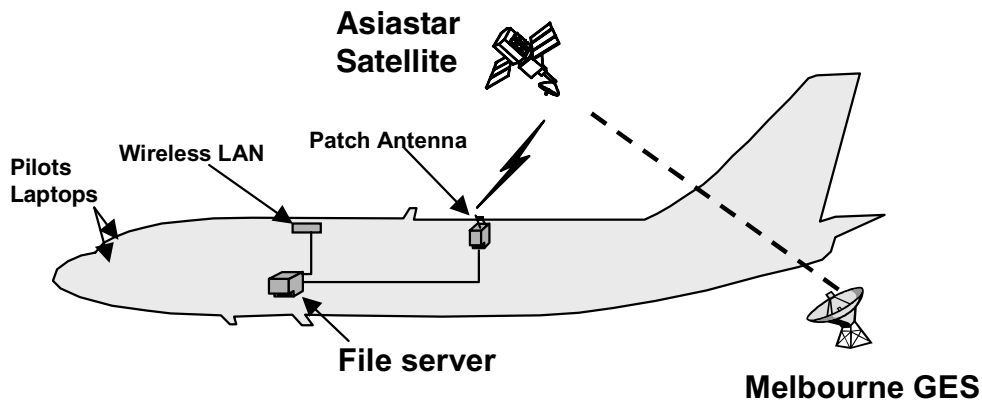
Figure 7 – SWIS Phase II on-board system configuration.
