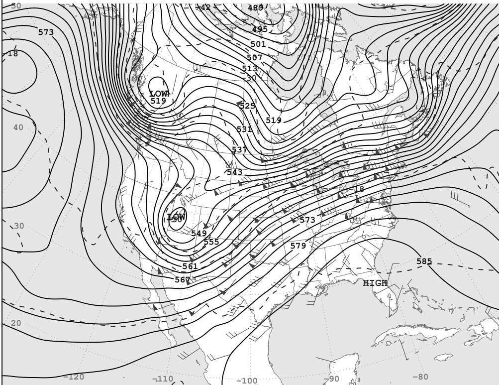
SAT, MAR 07, 2009 500-Millibar Height Contours at 7:00 A.M. E.S.T.
