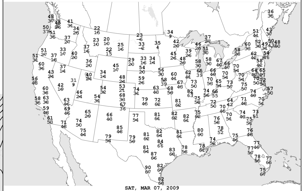
SAT, MAR 07, 2009 Highest and Lowest Temperature
