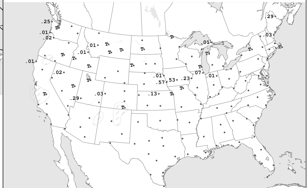
SAT, MAR 07, 2009 24-hour Precipitation Areas and Amounts Ending 7:00 A.M. E.S.T.
