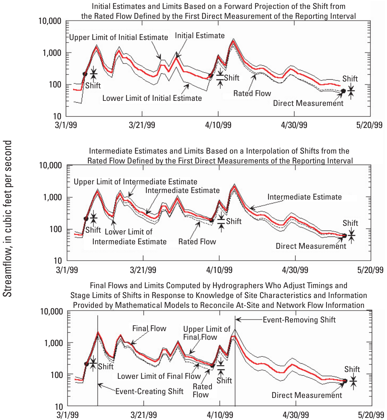
Figure 4. Hydrograph showing relation between shifts in the rated streamflow defined by direct measurements, initial and intermediate estimates, and final streamflow computations.
