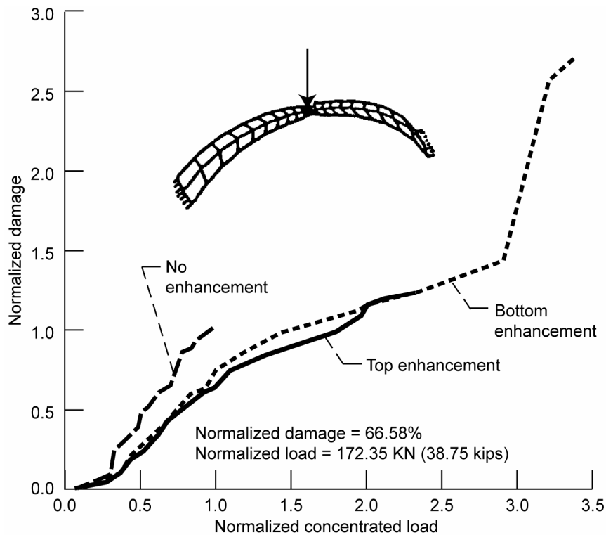
Figure 10.—Progressive structural fracture of a concrete-reinforced arch with and without composite enhancements.
