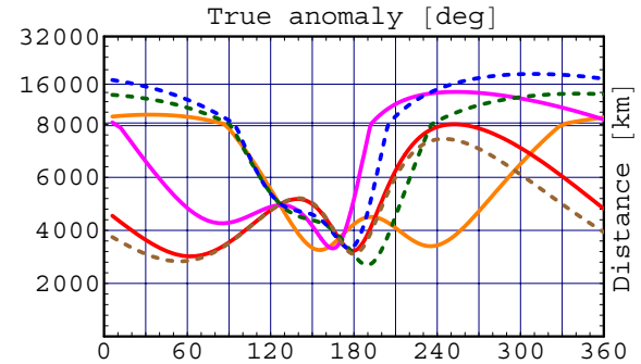
Figure 6 S/C interdistance plots. Sept. 2002
