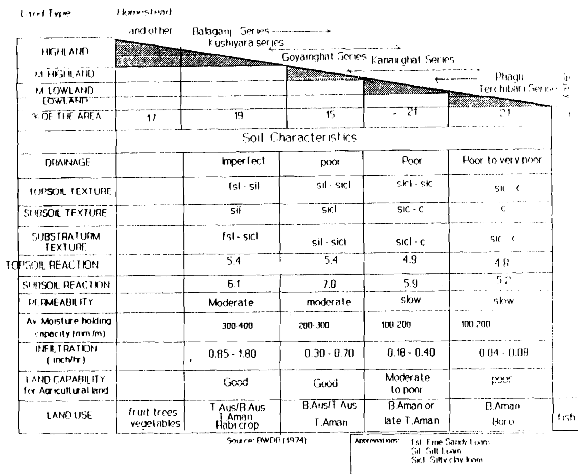
Figure 5.10. Relationship of soils to topography and hydrology in the Surma-Kushiyara project area.
