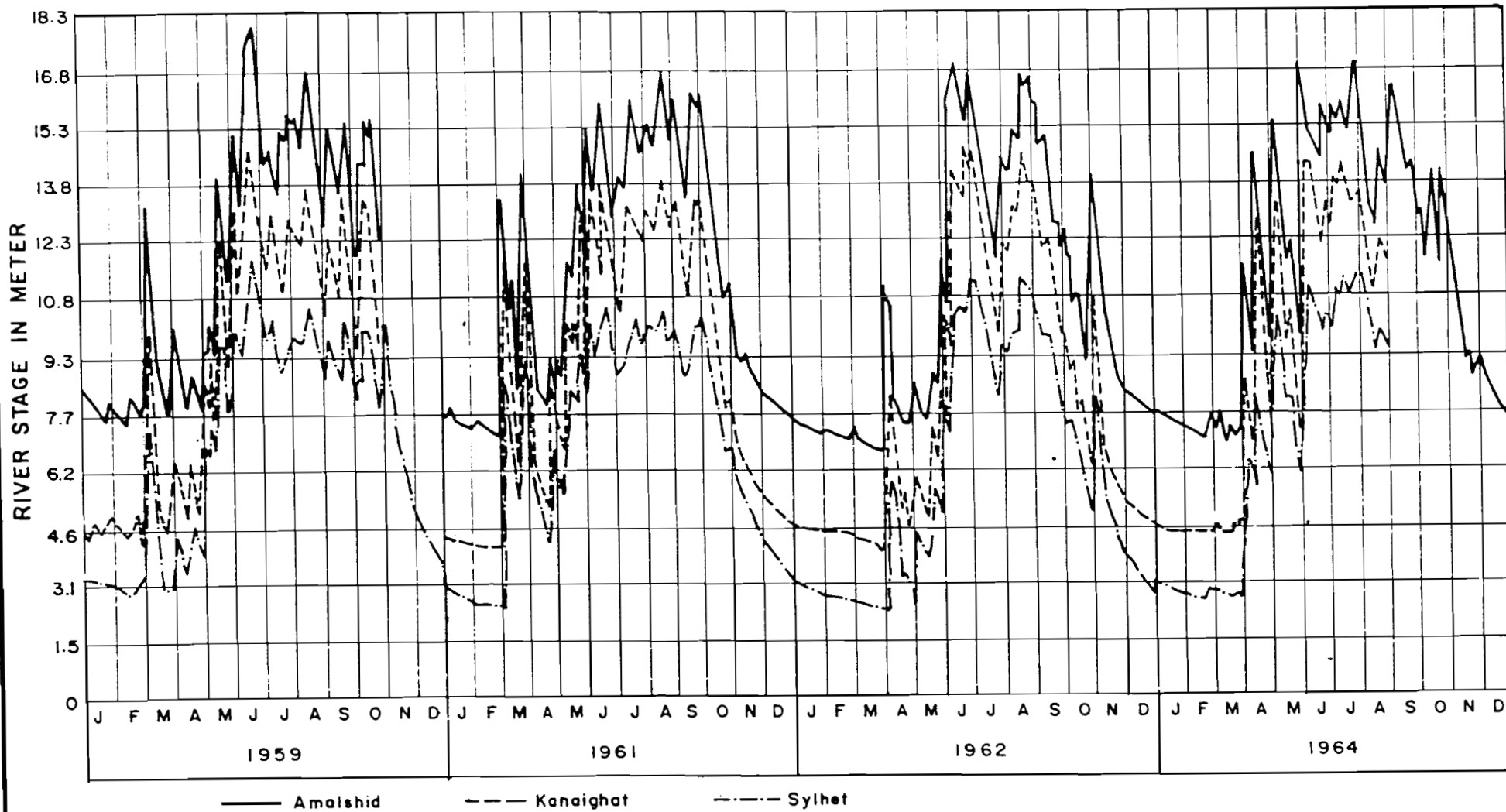
Figure 5.5 River stage hydrographs of the Surma River, 1959, 1961, 1962 and 1964
