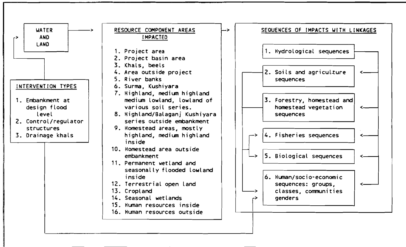
Figure 7.2. Cause and effect sequences: Surma-Kushiyara area with full-flood protection
