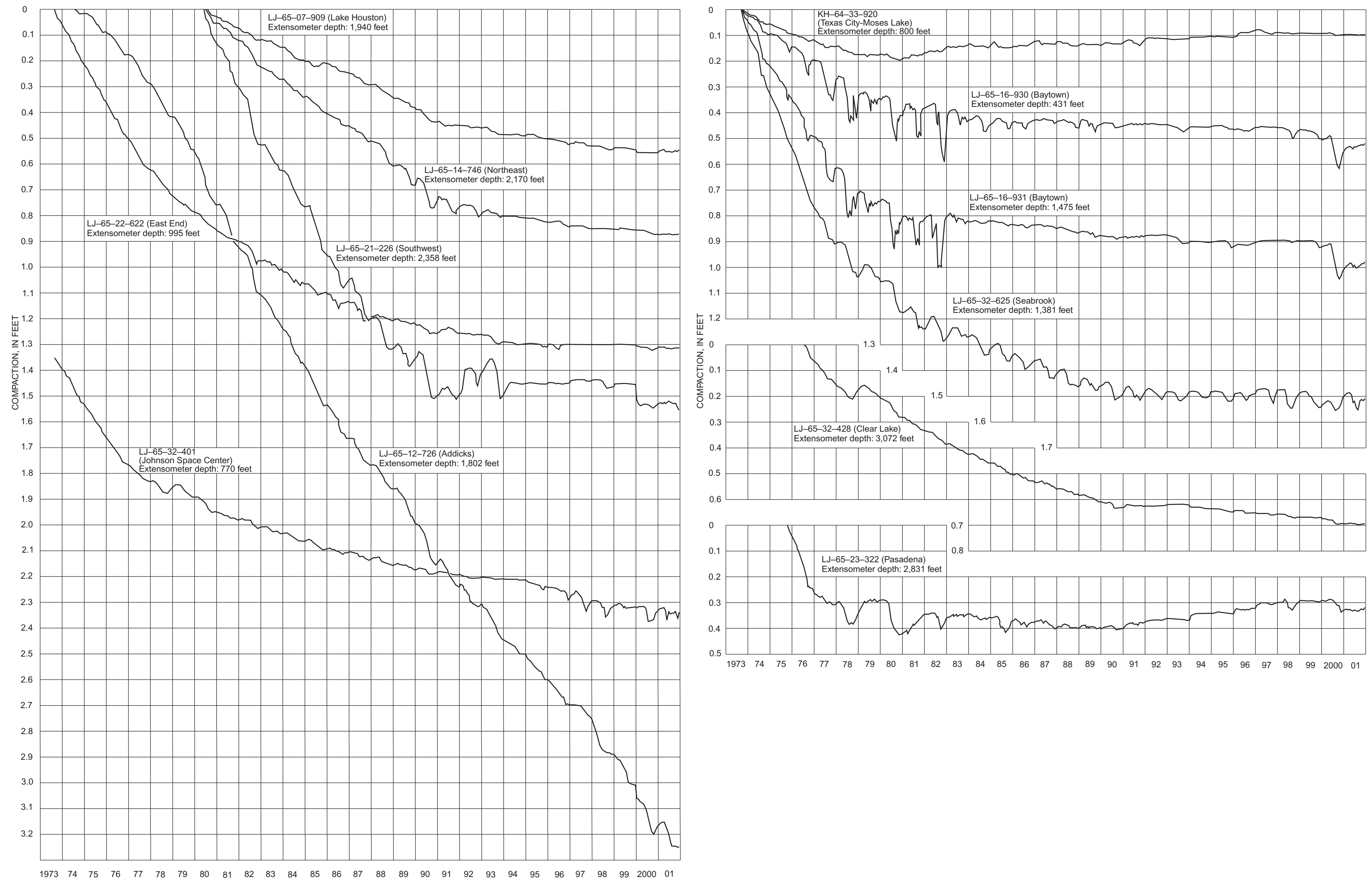
Figure 15. Graphs showing measured compaction of subsurface material, 1973-2001, at extensometer sites shown in figure 14.
