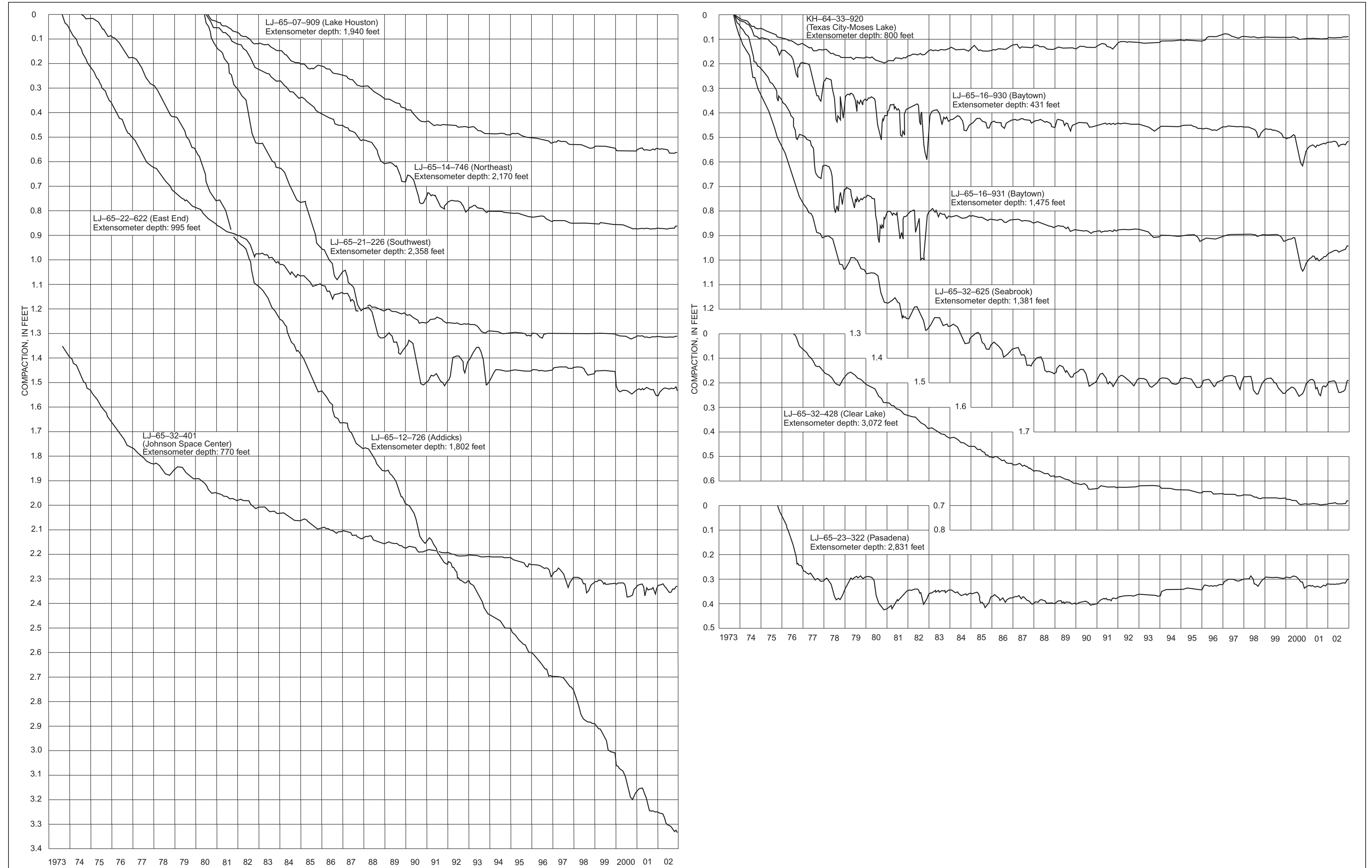
Figure 15. Graphs showing measured compaction of subsurface material, 1973-2002, at borehole extensometer sites shown in figure 14.
