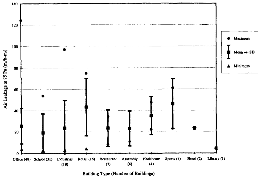
Figure 4 Airtightness values grouped by building type.
