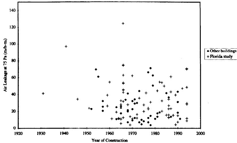
Figure 1 Airtightness vs. year of construction.
