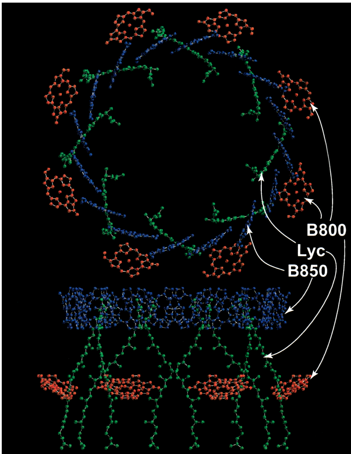
Figure 1. Top and side view of pigments in the Light Harvesting Complex II (LH2) of Rs. molischianum . The aggregate is made of the upper ring of 16 Bchls- a (blue) paired in 8 \alpha\beta heterodimers or intrasubunits (B850 molecules), lower ring of 8 Bchls- a (red) (B800 molecules), and ring of 8 lycopenes (carotenoids) (green).
