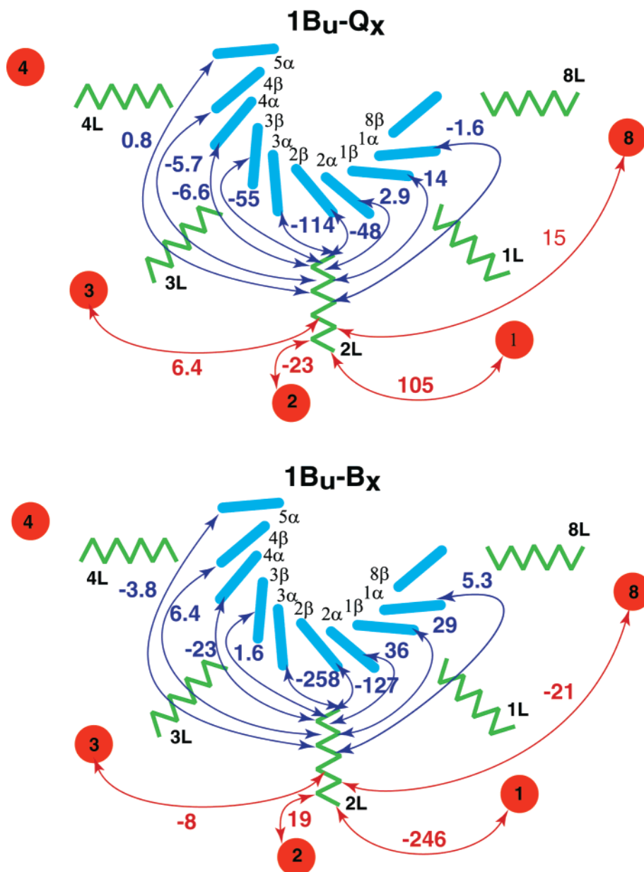
Figure 5. Graphical representation of the calculated excitonic couplings (in \text{cm}^{-1} ) in LH2 of Rs. molischianum shown in Figure 1 in the dielectric medium. These couplings are also given in Table 4.
