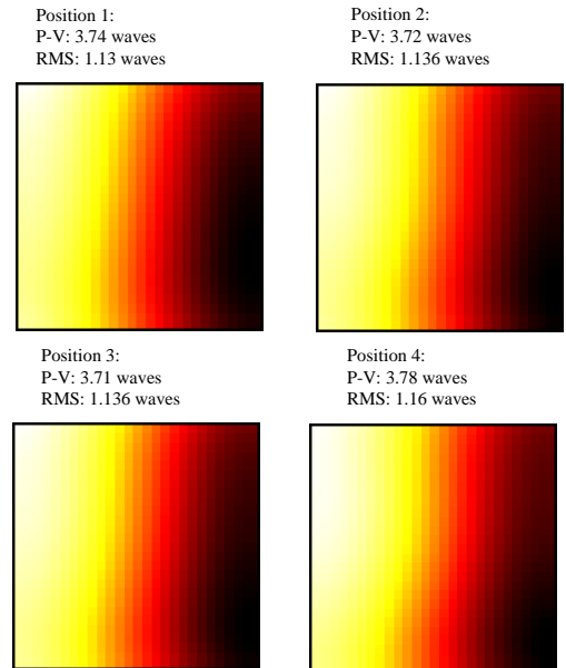
Fig. 2. Results of time dependent phase front measurements. The horizontal axis is in the zigzag plane.
