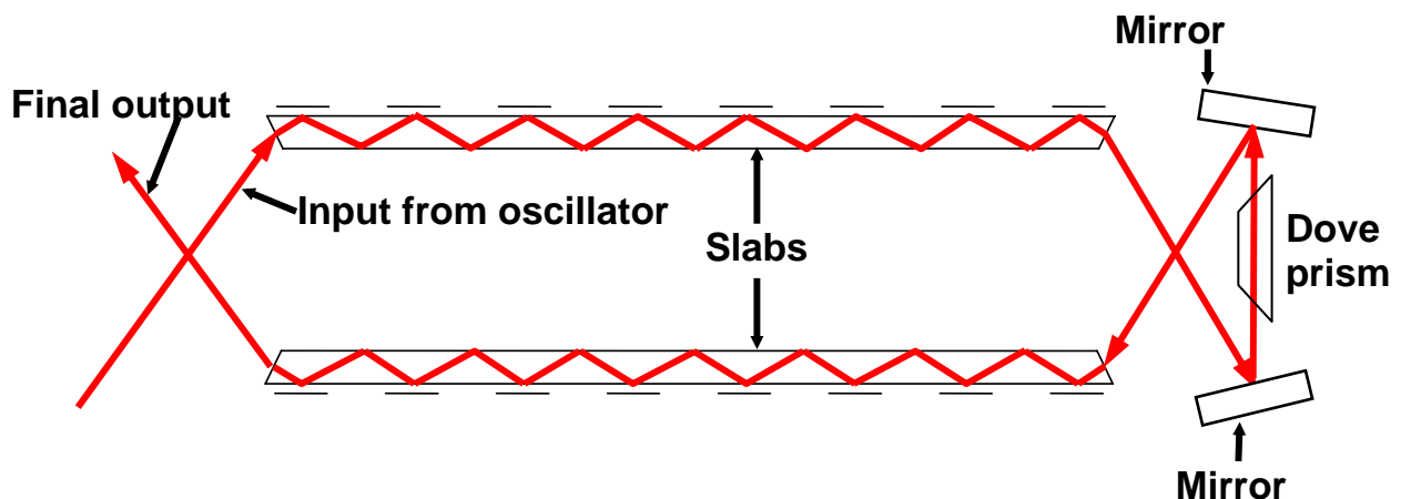
Figure 10. Final Phase II amplifier design
