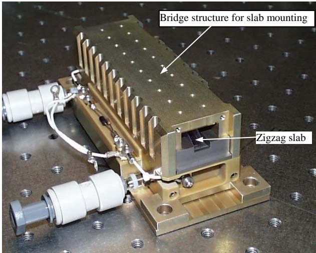
Fig. 1. Conductively cooled laser head.
