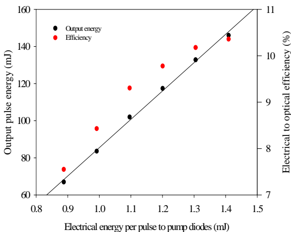
Figure 7. Unstable ring optical output vs. electrical input for 50 Hz operation
