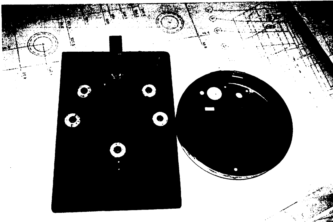
Top photo shows cover next to jig it fits over. Bottom photo shows cover in place on jig. Clips on cover can be seen in open spaces on jig.
