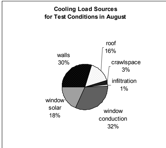
Figure 5. Cooling Load Sources under Unoccupied Test Conditions in August
