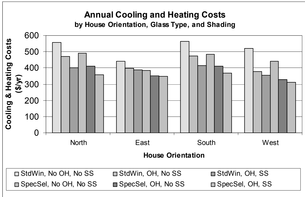
Figure 8. Annual Cooling and Heating Costs by Orientation, Glass Type (StdWin = standard glazing, SpecSel = spectrally-selective), Overhangs (OH), & Site Shading (SS)
