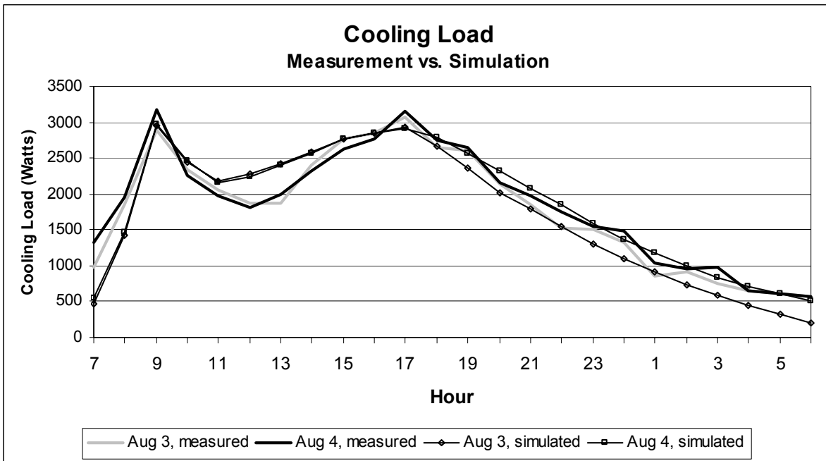
Figure 3. Daily Profiles of Cooling Load for Measured and Simulated Results
