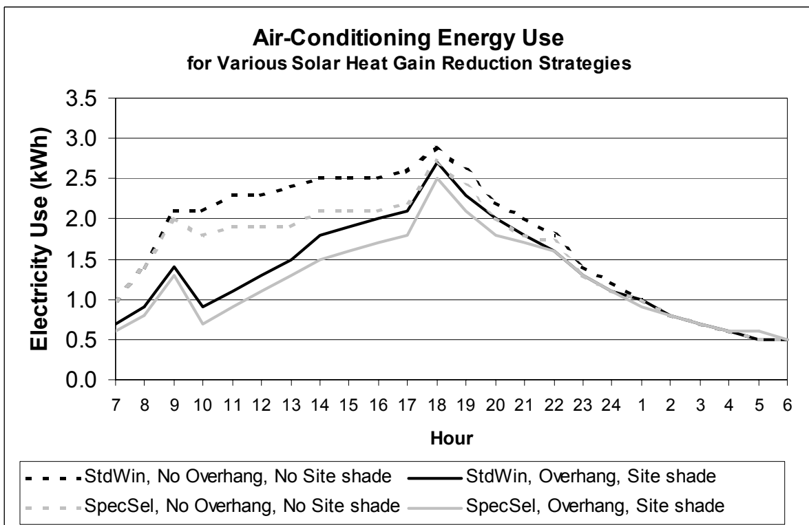
Figure 7. Daily Load Profiles Comparing Standard Windows (StdWin) with and without Shading, and Spectrally Selective Windows (SpecSel) with and without Shading
