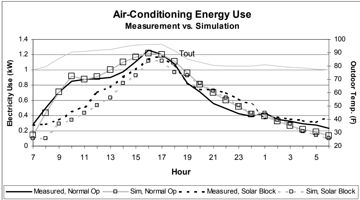
Figure 4. Daily Profiles of Air-Conditioning Energy Use for Measured and Simulated Results
