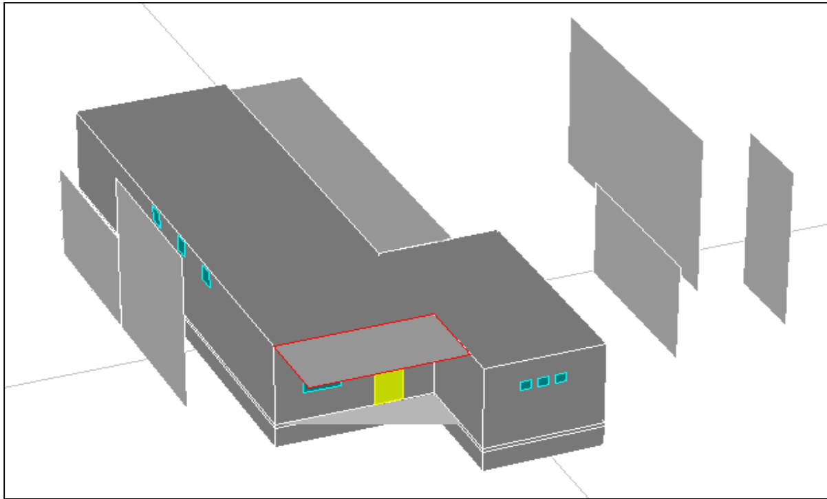
Figure 2. Building Geometry, View from Southwest with Overhangs and Site Shading
