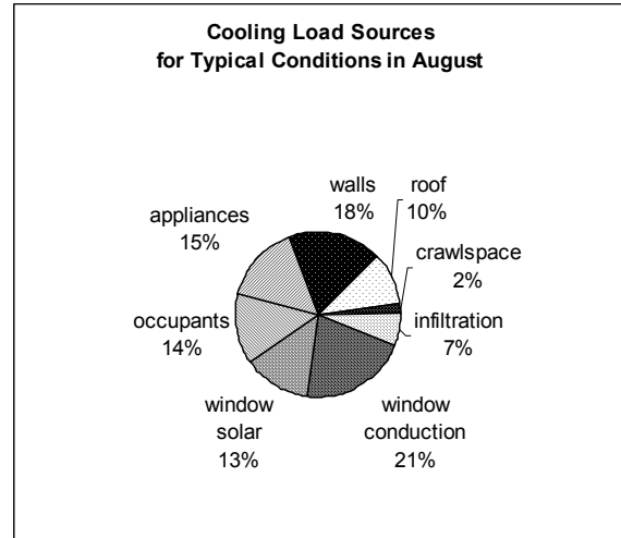
Figure 6. Cooling Load Sources under Simulated Occupied Conditions in August
