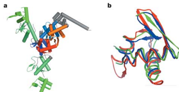
Figure 2 Winged helix folds in ESCRT-II. a , WH folds are highlighted in light and dark blue (Vps22 WH1 and WH2), light and dark green (Vps25 WH1 and WH2), and orange and red (Vps36 WH1 and WH2); the rest of the structure is coloured grey. b , Superposition of WH2 of Vps22, WH2 of Vps36 and WH2 of Vps25. Colours are as in Fig. 1.
