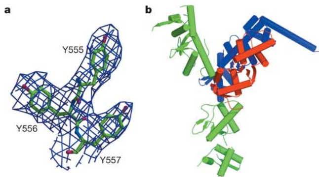
Figure 1 Structure of the ESCRT-II complex. a , Electron density from solvent-flattened SIRAS map contoured at 0.7 σ in the vicinity of the Vps25–Vps36 interface showing the refined structure in a stick model for Vps36 Tyr 555, Tyr 556 and Tyr 557. b , Overall structure of the complex: Vps22 is blue, Vps36 red and Vps25 green.
