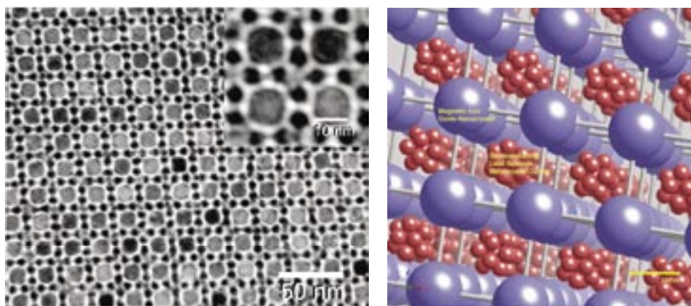
Figure 3.15. Transmission electron micrograph of bimodal nanocrystal superlattice (left). Schematic diagram showing components of a binary nanomaterial superlattice (right) [56].
