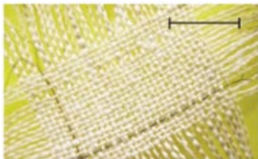
Figure 3.14. Photograph of a textile containing two nanotube-fiber supercapacitors woven in orthogonal directions. Two nanotube composite fibers were separately coated with electrolyte by dipping in aqueous polyvinyl phosphoric acid (19% phosphoric acid and 4% polyvinyl alcohol by weight), twisted together.
