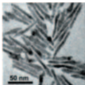
Transmission electron micrographs of cadmium selenide nanocrystals used in a photovoltaic device. Tuning the size and aspect ratio of the nanocrystals gives control over the band gap and electron transport distance. External quantum efficiencies of over 54% have been achieved [Courtesy of A.P. Alivisatos, Univ. of California, Berkeley and Lawrence Berkeley National Laboratory].
