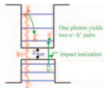
Enhanced Photovoltaic Efficiency in Quantum Dot Solar Cells by Inverse Auger effect (Impact Ionization) [Courtesy of V. Klimov, Los Alamos National Laboratory].
