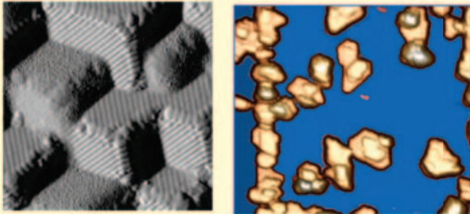
Left: STM image of faceted Pd/W(111) (15 nm x 15 nm) – rows of individual atoms are visible on the flat faces of the three-dimensional nanoarchitecture of a faceted W surface. Right: STM image (200 nm x 200 nm) – ruthenium nanoparticles on graphite substrate [Courtesy of T. Madey, Rutgers Univ., and J. Hrbek, Brookhaven National Laboratory].
