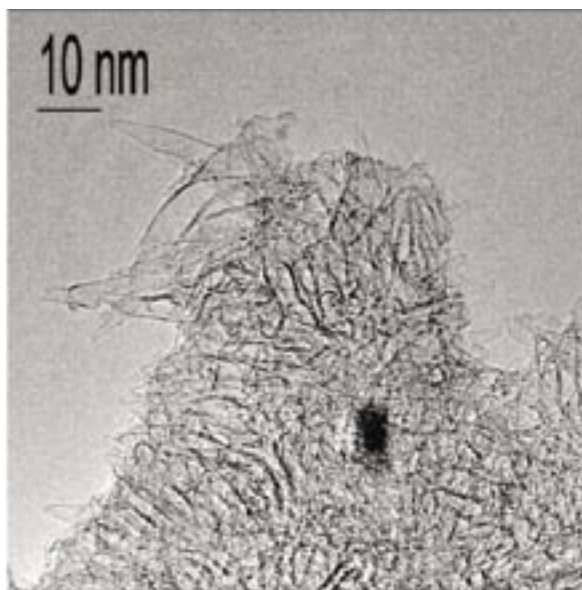
Figure 3.19. Carbon nanohorn aggregate formed by high-power laser vaporization [Courtesy of D.B. Geohegan, Oak Ridge National Lab].
