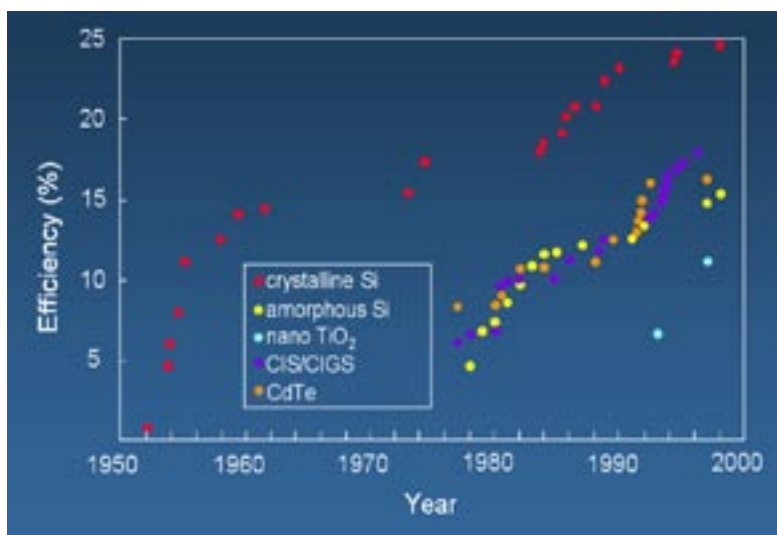
Figure 3.6. Efficiency of photovoltaic devices [32].
