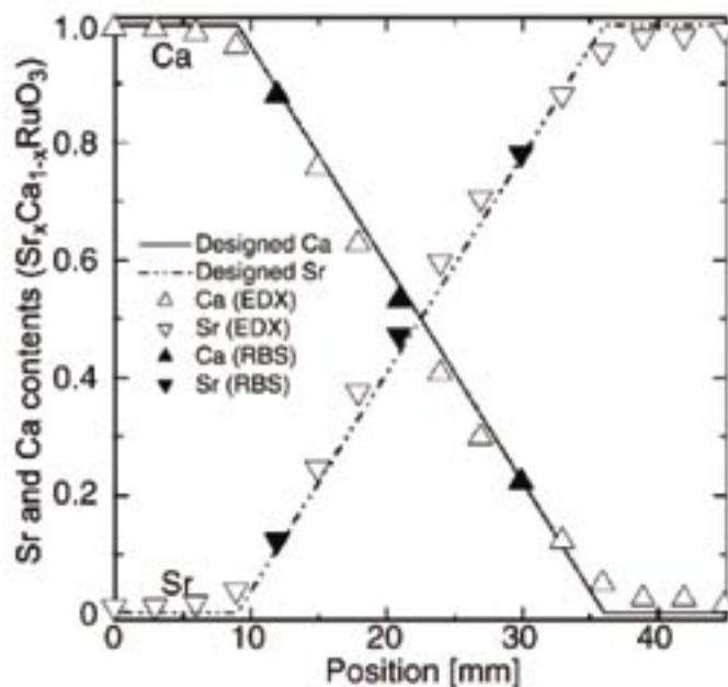
Figure 3.18. Sr and Ca compositions of a \text{Sr}_x\text{Ca}_{1-x}\text{RuO}_3 composition-spread film, plotted as a function of substrate position, as determined by EDX and RBS. Excellent agreement is obtained between designed and actual compositions [61].
