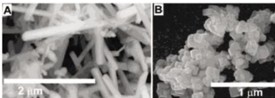
Figure 3.17. Solid-state synthesis of perovskite nanoparticles. A. \text{BaTiO}_3 nanorods, B. \text{SrTiO}_3 nanocubes [59].
