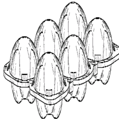
Example of a design for compartmented type packaging for egg or ball shape.
