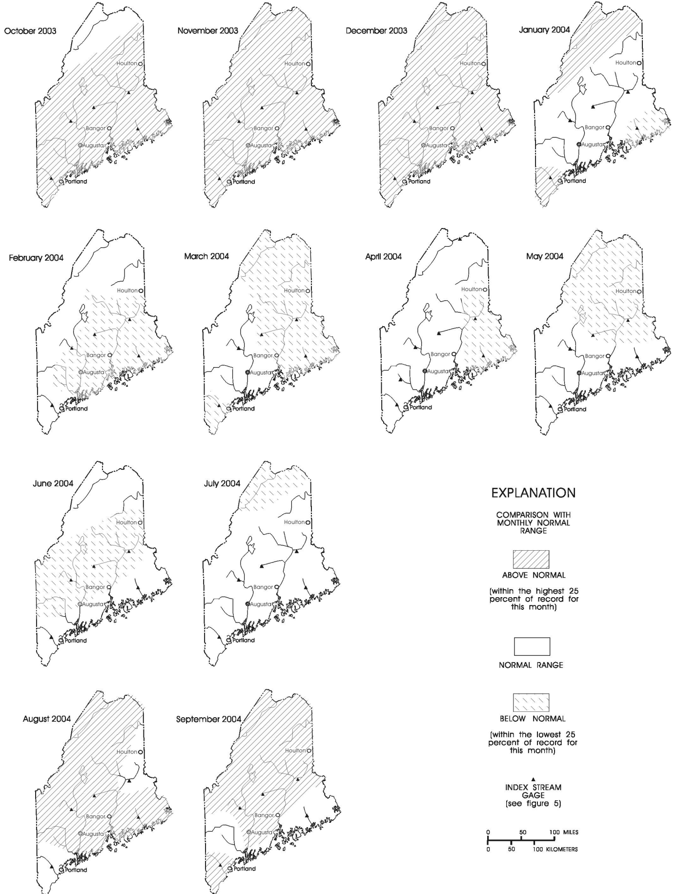
Figure 6.--Monthly surface-water conditions during the 2004 water year in Maine.
