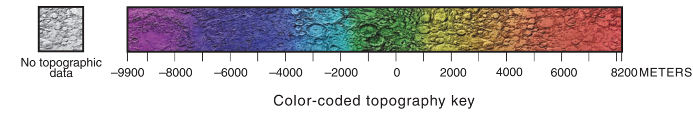
LAC 62 Scale 1:1,000,000 Mercator Projection
