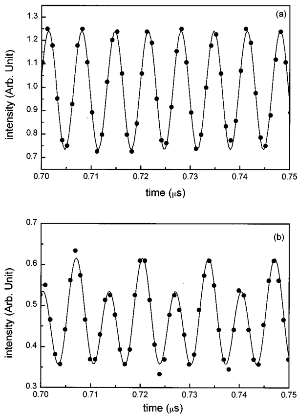
FIG. 6. A portion of a measured ( \bullet ) ring-down signal providing evidence of longitudinal and transverse mode beating in a confocal cavity when the detector was (a) unobscured and (b) partially blocked. The solid lines in both figures represent best-fit sine waves with beat frequencies of 150 MHz and 75 MHz. In (a), only beating at the longitudinal mode spacing, \nu_f=150 MHz is evident, whereas in (b) frequencies at both the longitudinal and transverse mode spacings of 150 MHz and 75 MHz, respectively, are observed.
