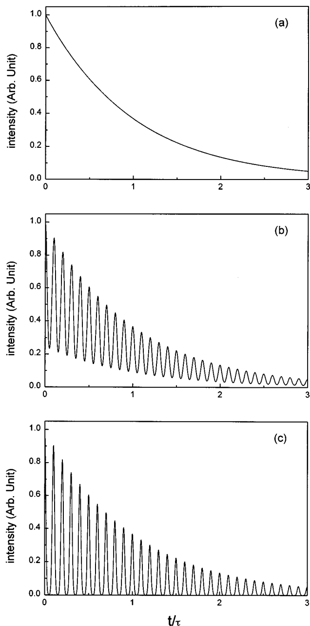
FIG. 2. Ring-down signals calculated using Eq. (21) for (a) “short,” (b) “intermediate,” and (c) “long” cavity cases for transform-limited pulses with \eta=0.1, 0.75, and 1.25, respectively. For these calculations, the excitation spectrum was centered on a cavity eigenfrequency.
