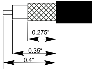
CABLE STRIPPING DIMENSIONS
