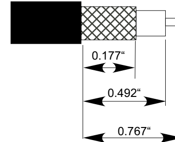
CABLE STRIPPING DIMENSIONS
