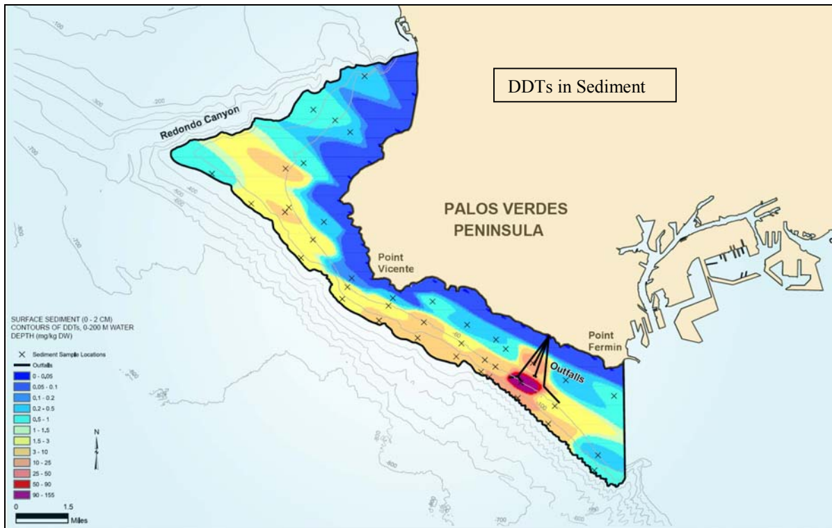
Figure 1-1 Sediment Concentrations near Palos Verdes Shelf
