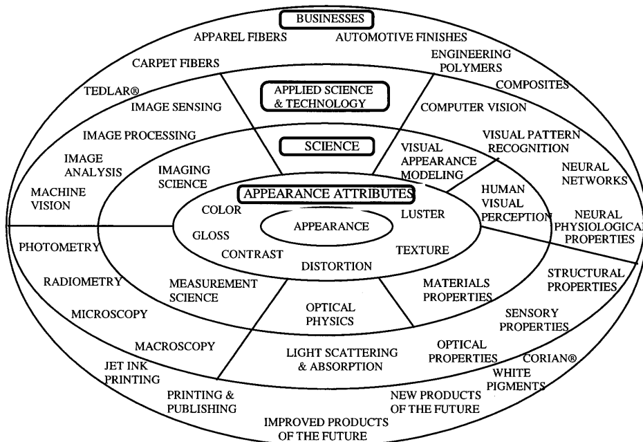
Fig. 1. Connectivity of areas and groups involved in appearance measurements (P. Tannenbaum et al.)
