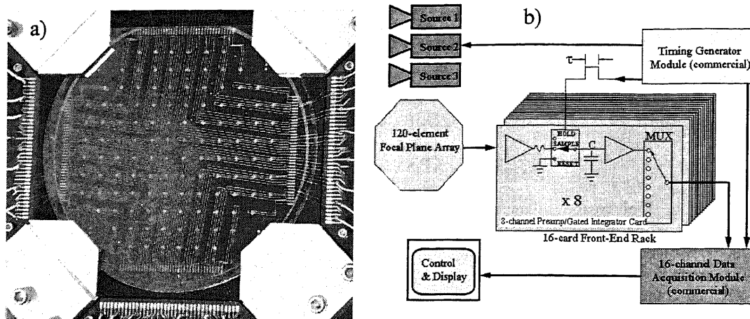
Fig. 1: a) The 120-element antenna-coupled microbolometer focal plane array. The wafer diameter is 75 mm. b) The system architecture. See text for explanation.
