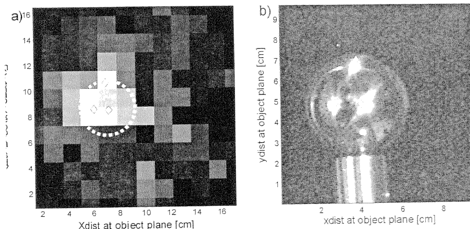
Fig. 4. a) An active mm-wave image of a steel bearing. The Gaussian fit centroids to the image indicate the location of the reflections. The dashed circle indicates the outline of the bearing. b) An optical image of the bearing from the on-axis video camera. Three bright optical reflections indicate the positions of the sources. The diamonds mark the source positions determined from the mm-wave image. Note the slightly different axis for the two figures. The maximum signal level in this image is better than 2000\sigma ; the lit pixels outside the location of the bearing are likely due to audio frequency crosstalk between channels.
