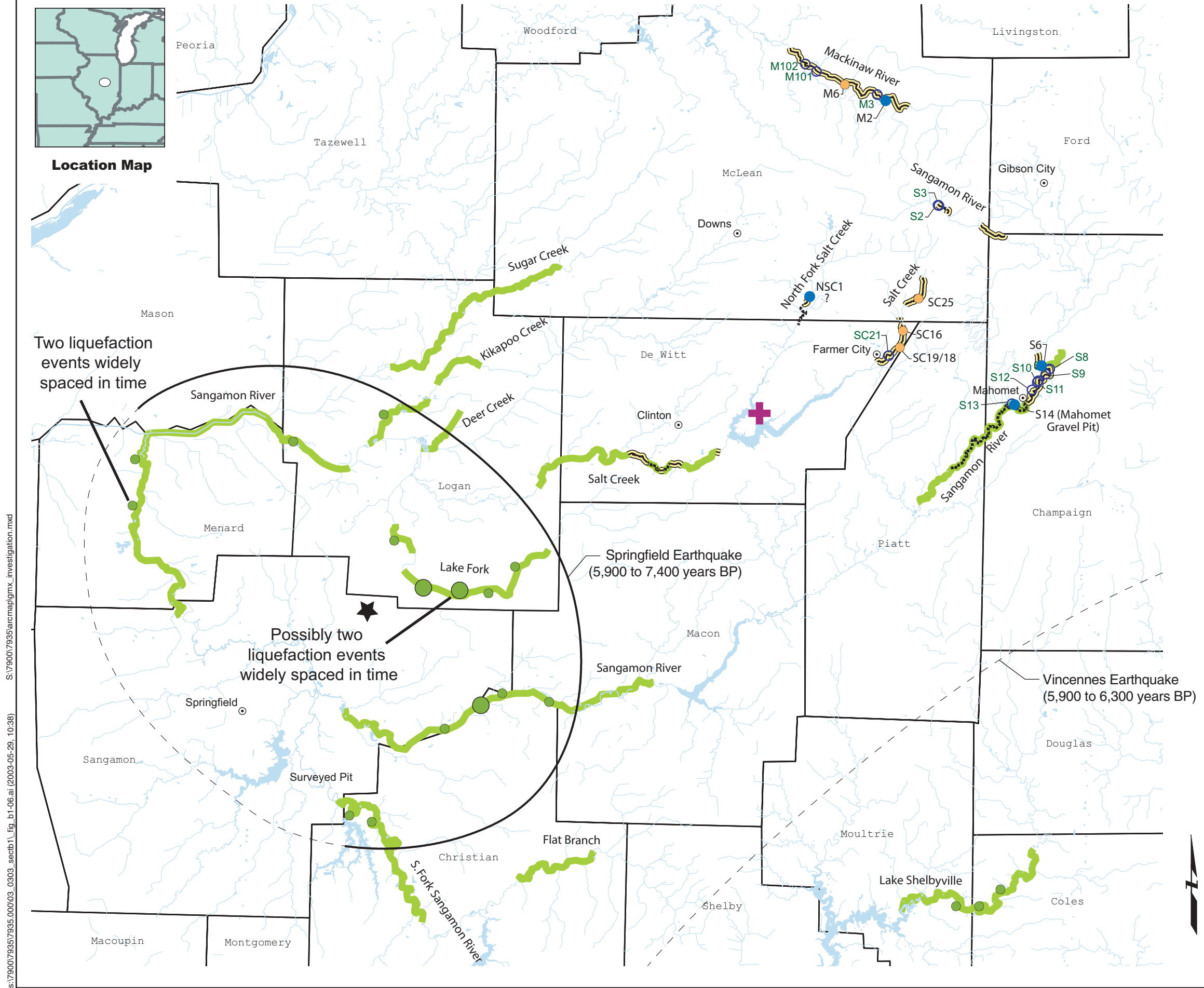
Figure B-1-6 Seismic Hazards Report for the EGC ESP Site Map Showing Surveyed Stream Banks and Evidence for Paleoliquefaction in the Site Vicinity
