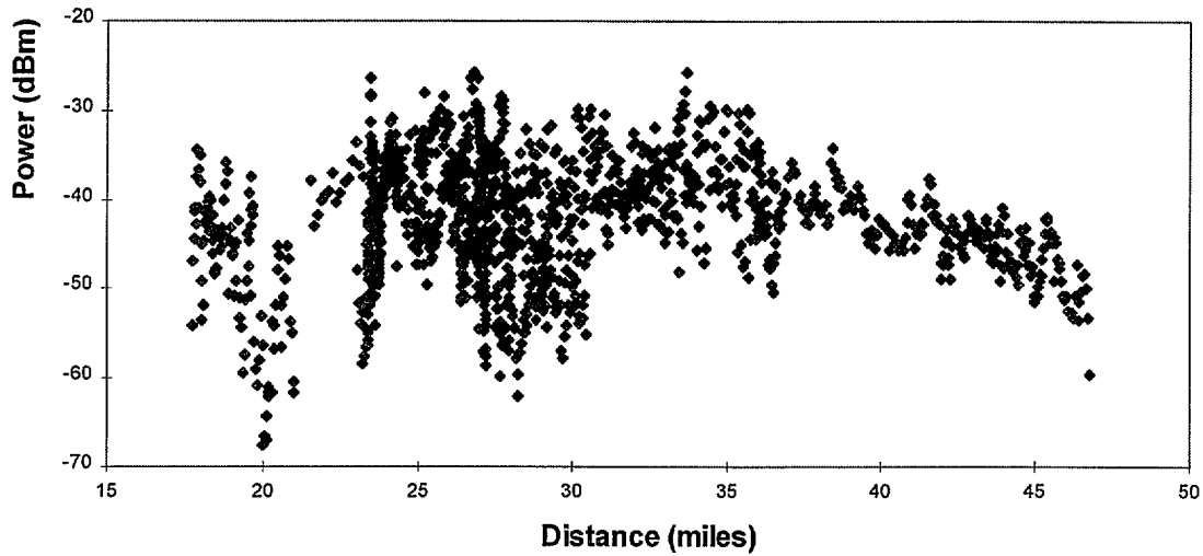
Figure 41. Received signal power vs. distance from transmitter for urban low-rise environment.
