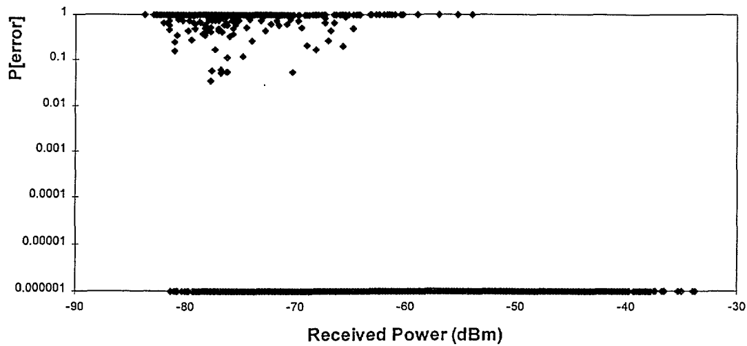
Figure 16. Packet error rates vs. received signal power for rural plains environment.
