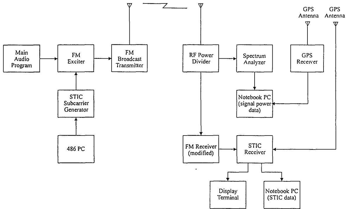
Figure 5. STIC field test configuration.
