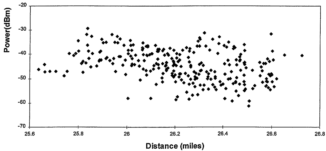
Figure 52. Received signal power vs. distance from transmitter for urban high-rise environment.
