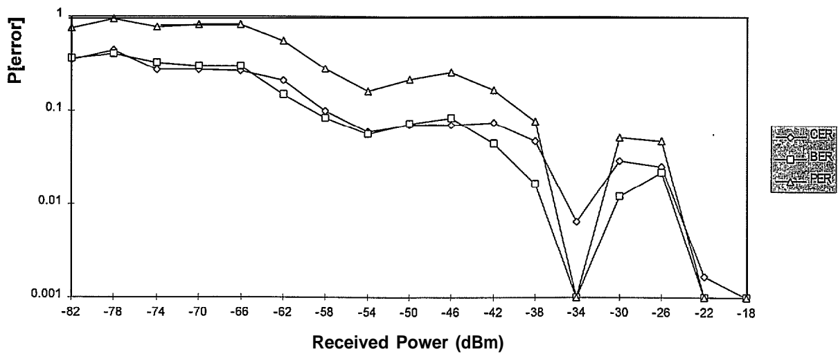
Figure 21. Mean CER, BER, and PER vs. received signal power (SYNC data) for rural mountain environment.
