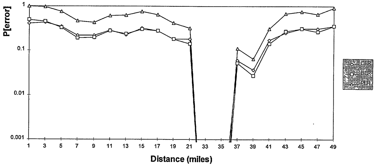
Figure 25. Mean CER, BER, and PER vs. distance from transmitter for rural mountain environment.
