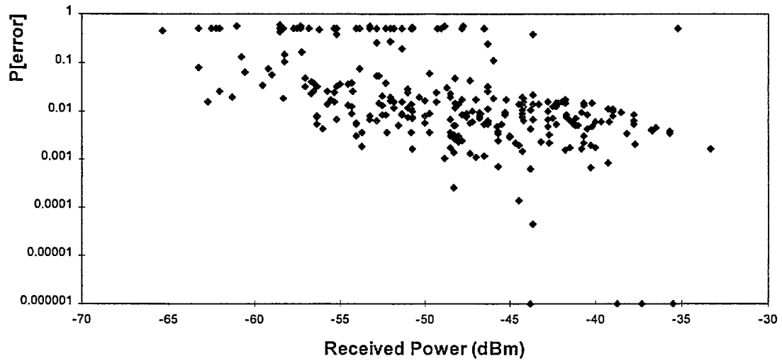
Figure 50. Channel error rates vs. received signal power for urban high-rise environment.
