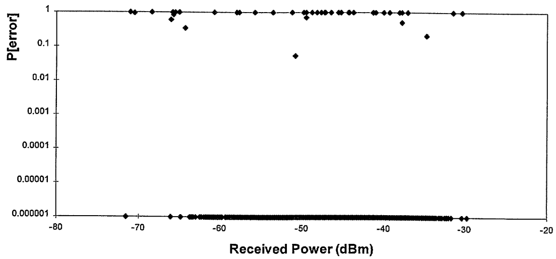
Figure 40. Packet error rates vs. received signal power for urban low-rise environment.
