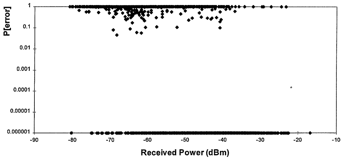
Figure 28. Packet error rates vs. received signal power for rural mountain environment.
