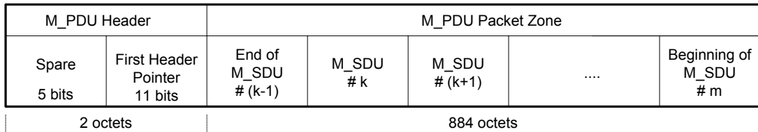
Figure 5. M_PDU Structure
