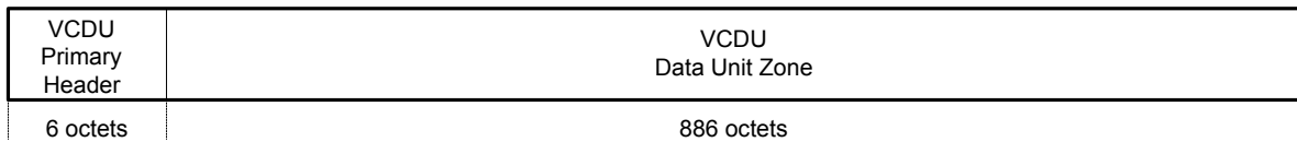
Figure 2. VCDU Structure
