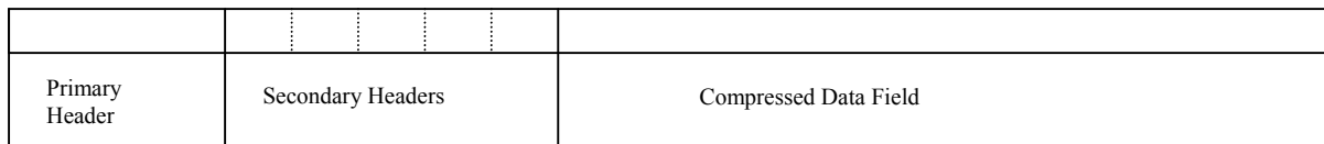
Figure 8. LRIT Session Protocol Data Unit (S_PDU)
