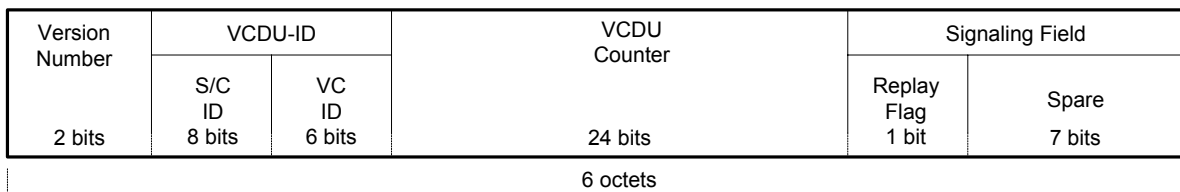
Figure 3. VCDU Primary Header
