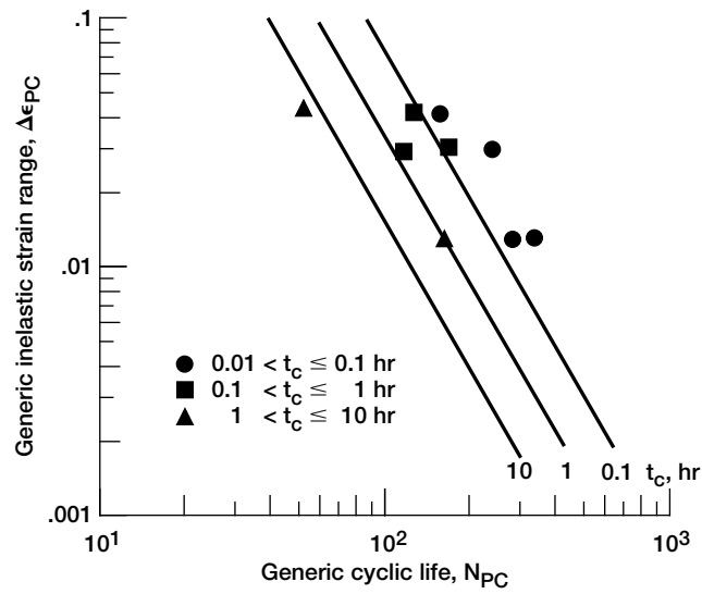
(b) PC type of loading.
