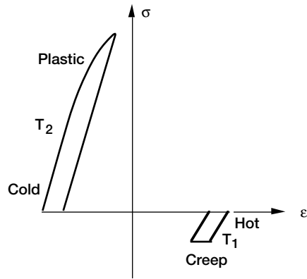
(e) Bithermal CCOP test.
