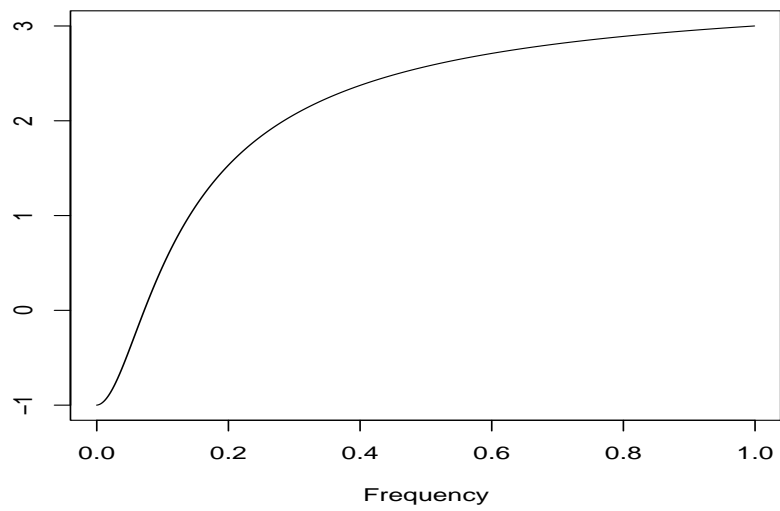
Figure 6: Phase Delay Function for the Forecast Filter
