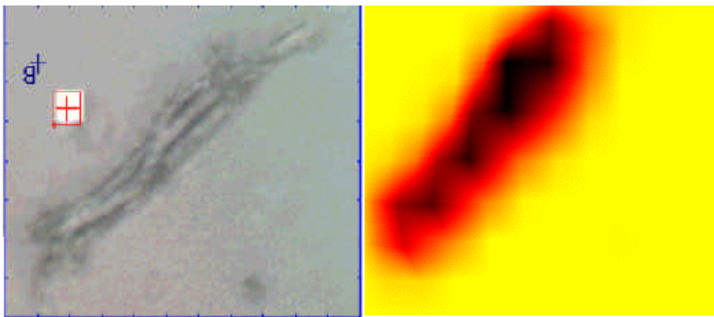
Figure 3. Chemical distribution of the protein characteristic bands amide I and amide II ( 1495\text{-}1800\text{cm}^{-1} ) of a Calothrix filament. a) Optical image, b) 2-D map of the protein distribution.
