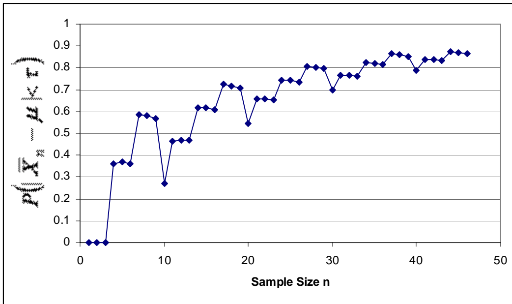
Figure 3. Plot of confidence level [P(\bar{X}_n - \mu < \tau)] vs Sample Size n. Length of CI: 2 \cdot \tau , \tau = .1 , and \text{Lambda} = .2
