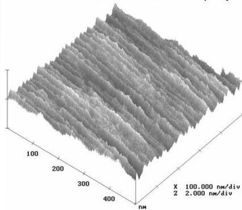
Commercial "Off-Axis" 4H-SiC Epilayer
