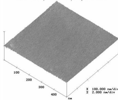
NASA "Step-Free" Epilayer Surface
