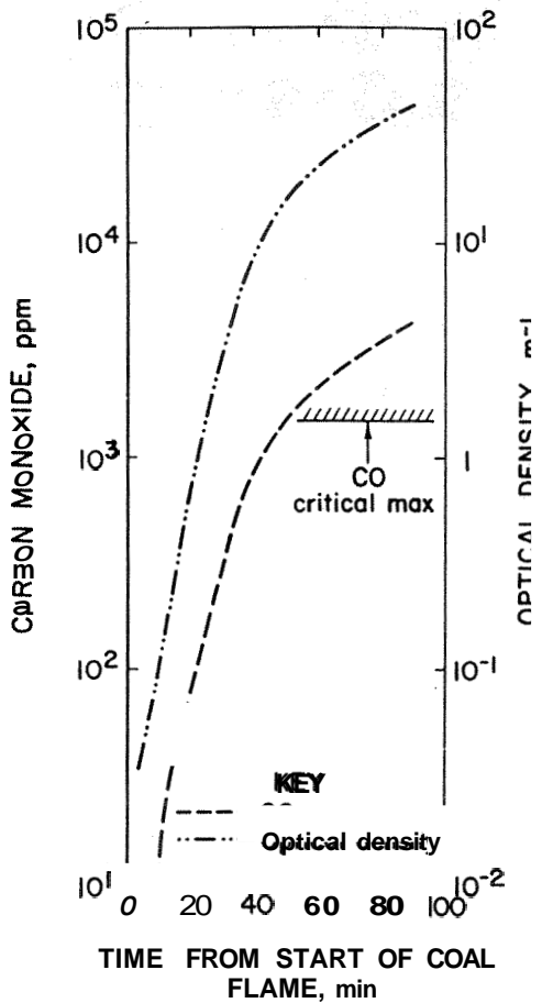
Fig. 1—Downstream carbon monoxide and smoke density levels during the growth of a typical SBR belt/coal test fire.
