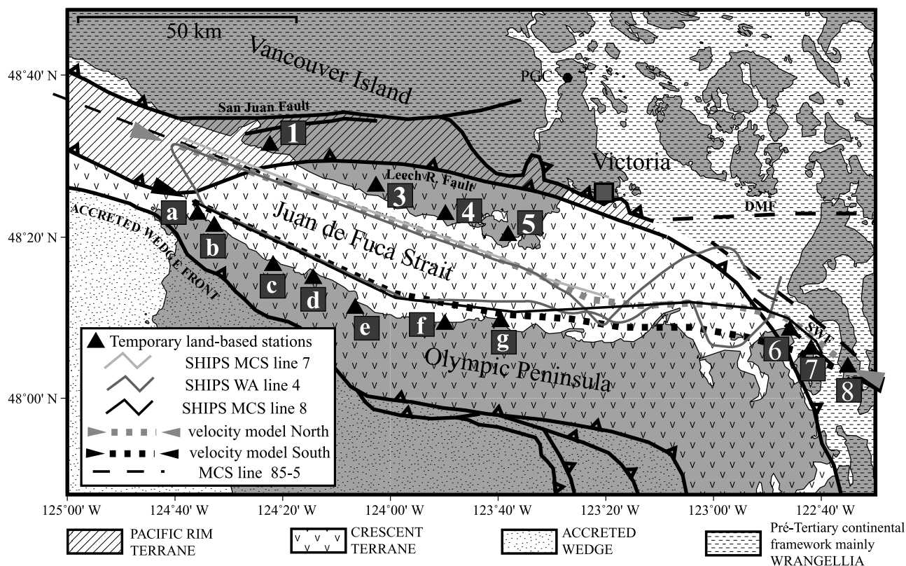
Figure 2. Principal geological units in study: accreted wedge, Crescent terrane, Pacific Rim terrane, and pre-Tertiary continental framework. The triangles are locations of land-based stations used in the travel time modeling of wide-angle arrivals. Shaded lines indicate MCS profiles, and ship track lines of the SHIPS indicate seismic reflection survey. DMF, Devils Mountain Fault; SWF, Southern Whidbey Island Fault.
