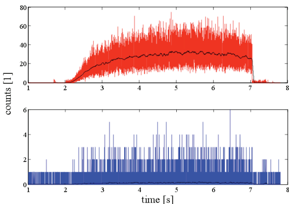
Figure 2: Spill-structure measurements with ^{12}\text{C}^{6+} at 430.10 MeV and 8 \cdot 10^7 p/spill. Top: IC. Bottom: BLM.
