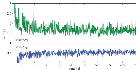
Figure 3: Ratios of Min and Max values divided by the average (5 ms integration window). Minimization of the interspace of both functions smooths the spill-structure.
