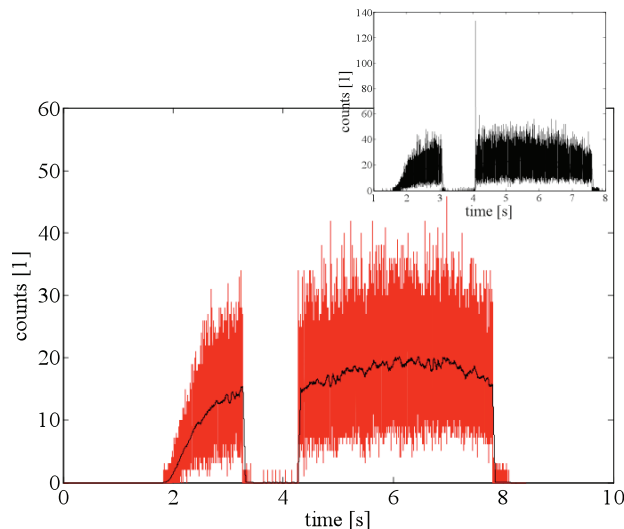
Figure 4: Slowly extracted ^{12}\text{C}^{6+} beam at 270 MeV with 1s spill-pause, 10 kSa/s. The black line is the result of a rolling average filter of 500 points window-size. Top right: spill with re-entry spike.
