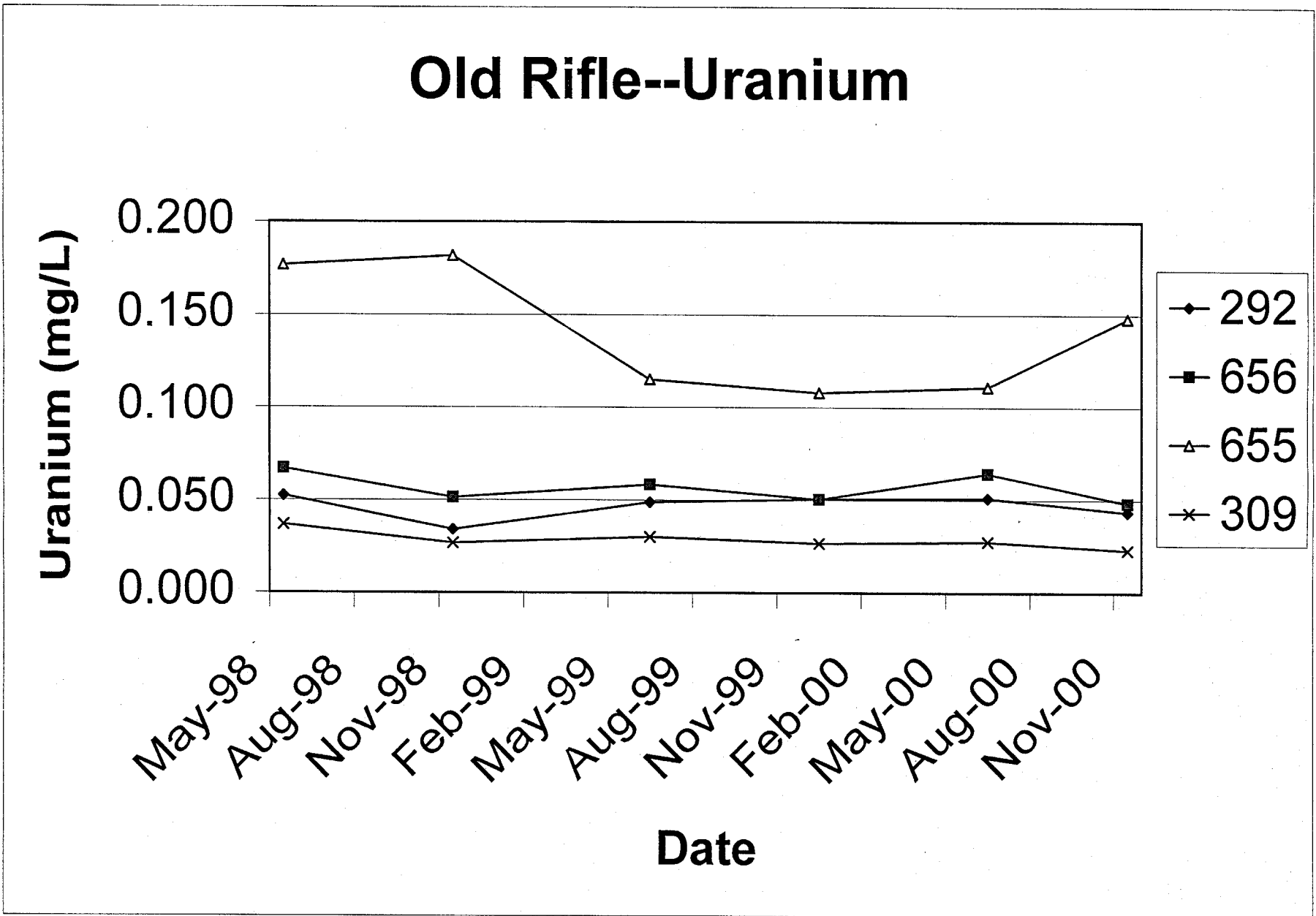
Figure 8. Time-Concentration Plot for Uranium for Old Rifle Wells 292, 309, 655, and 656
