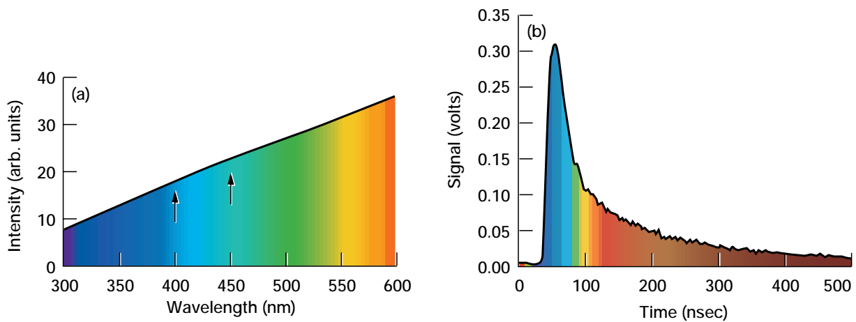
Figure 3.—(a) Spectrally resolved emission produced by the incandescing soot as a result of the pulsed laser heating. (b) Temporally resolved LII signal. The arrows indicate a commonly used spectral region for detecting LII.
