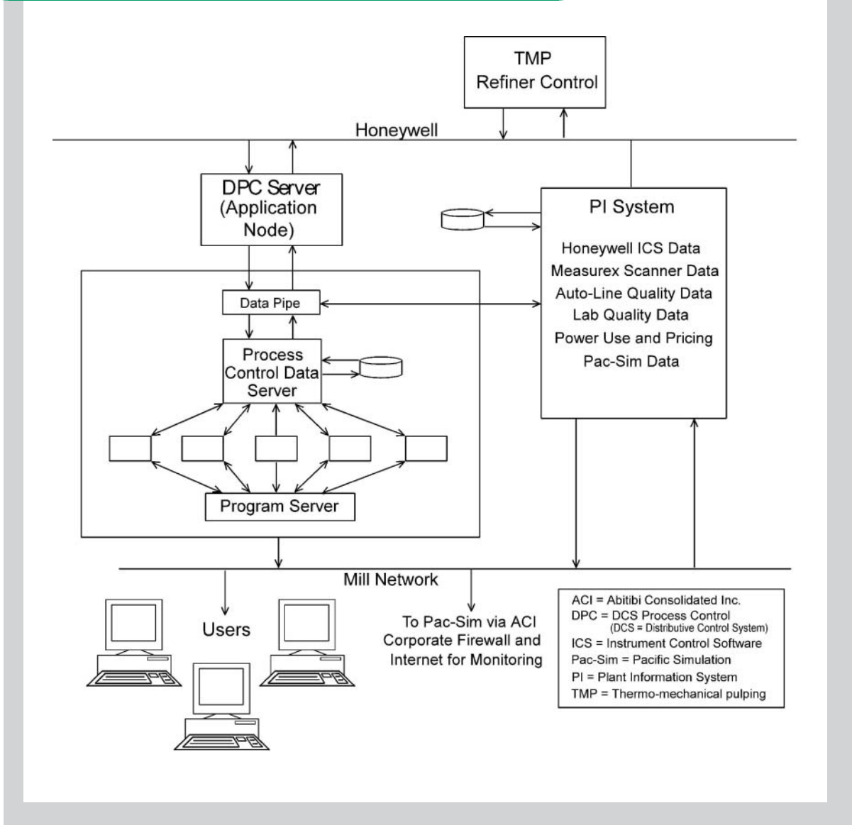
FIGURE 2. INSTALLED ADVANCED QUALITY CONTROL SYSTEM
